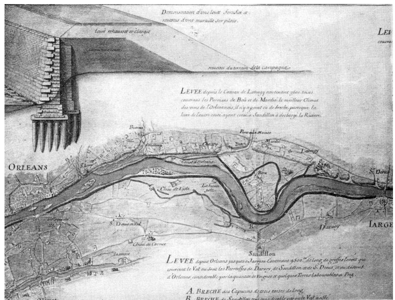
Figure 3.2 – Map and design of existing earth dams to be elevated in the early 1700s following a flood of the Loire river near Orléans, France, in 1709 (Dion, 1961).
