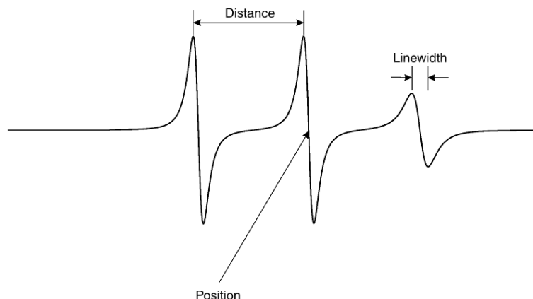
Figure 2.15 The EPR spectrum is characterized by the line positions, distances between lines, and linewidth.
