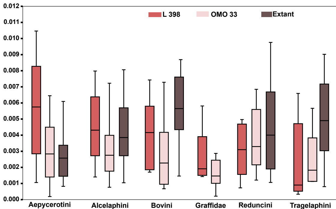
Figure 2. 11: Boxplots of epLsar (anisotropy) values for L 398, OMO 33, compared to extant bovid tribes. Note that the anisotropy values for OMO 33 are low.
