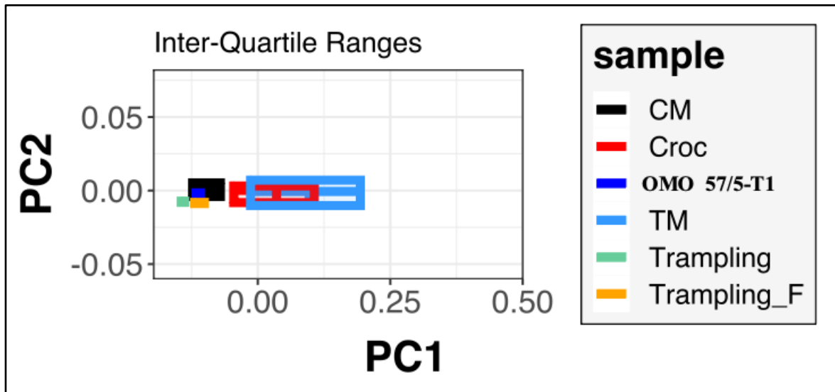
Figure 4. 11: PCA plots of Inter-Quartile Ranges shows OMO 57/5T1 overlap with the experimental cutmarks. CM (cutmark), Croc (crocodile bite mark), TM (Carnivoran tooth score), Trampling_F (trampling with flint).
