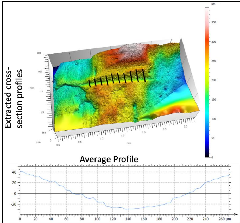
Figure 3. 3: Example of 3D model of a cutmark from a fossil specimen (OMO 377-T004) showing the position of the 10 cross sections (in black vertical lines), and an average profile of the extracted surfaces.
