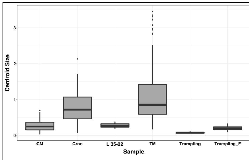
Figure 3. 18: Centroid size plot of BSM from L 35-22 (lower G) compared to experimental BSMs; cutmarks (CM), crocodile tooth scores (Croc), carnivoran tooth mark (TM), Trampling and trampling with flint (Trampling-F).
