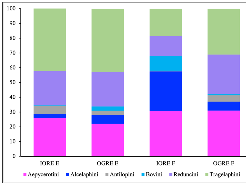
Figure 2. 4: Percentage counts of bovid tribes from members E and F collected by the IORE and the OGRE. The high number of Alcelaphini is visible only in IORE F. This is due to most of the bovid samples for the IORE Member F comes from unit F-0, in particular from large scale excavations carried out at L 398 and OMO 33 by the IORE.
