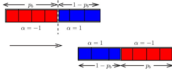
Figure 6.3: The array on the left is X_b ( b 's neighbors in \vec{x} in decreasing order of b 's preference) and the array on the right is X'_b .
