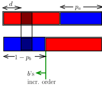
Figure 6.4: The top array is X'_a and the darkened cell there contains b . The cell exactly below this in the blue sub-array of X'_b contains a .
