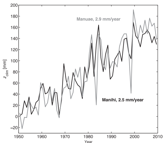
Figure 4. Reconstruction of the climatic component of historic sea-level ( z_{\text{clim}} ) since 1950 (data from the analysis of Becker et al. , 2012), indicating the estimated linear sea-level rise trends at Manihi (black) and Manuae (gray).
