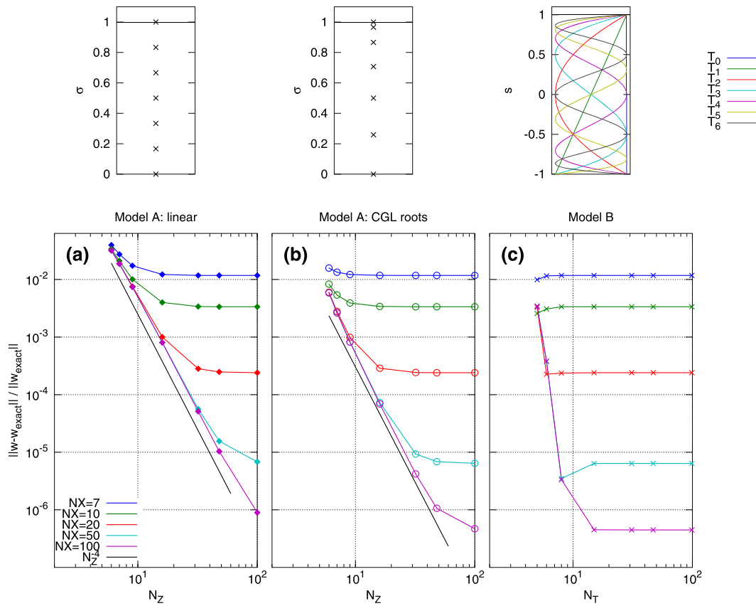
Figure 1. Convergence of the vertical velocity at the free surface \tilde{w} for Models A and B, for a linear wave with kh \sim 4 . The convergence is evaluated as a function of N_x , N_z , and the vertical resolution: (a) Model A: linear distribution, (b) Model A: roots of Chebyshev–Gauss–Lobatto (CGL) polynomials, and (c) Model B: spectral method. In the top row, examples of both of the vertical point distributions are shown for Model A (with N_z = 7 ), and of the Chebyshev polynomials for Model B (with N_T = 6 ).
