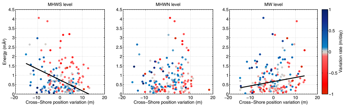
Fig. 6 Erosion (red)/accretion (blue) rate as a function of the to cross-shore position and wave energy ( m^2 ) for: Left MHWS, Center MHWN and Right MW levels; linear equilibrium functions are fitted for variation rates included in [-0.05; 0.05] m/day (black lines)
