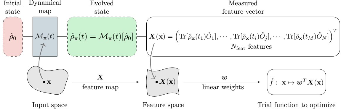
Figure 5.1: General scheme of constructing a reservoir-computing trial function \hat{f}(\mathbf{x}) using a physical system. The system, prepared in a fixed initial state \hat{\rho}_0 , is subjected to a time evolution depending on the input \mathbf{x} . This dependence can be realized, for example, via some kind of driving on the system determined by \mathbf{x} , such as considered in [8]. We formally denote this time evolution with the dynamical map \mathcal{M}_{\mathbf{x}}(t) , which gives the state of the evolved physical system at a later time: \hat{\rho}_{\mathbf{x}}(t) = \mathcal{M}_{\mathbf{x}}(t)[\hat{\rho}_0] . During this time evolution, a set of observables \{\hat{O}_i\}_i are measured at different times \{t_j\}_j . [We assume ensemble measurements for quantum systems, such that we can measure the expectation values of multiple (possibly noncommuting) observables.] The input \mathbf{x} is therefore transformed into a feature vector \mathbf{X}(\mathbf{x}) containing N_{\text{feat}} features of the form \text{Tr}[\hat{\rho}_{\mathbf{x}}(t_j)\hat{O}_i] (the order does not matter). Finally, the trial function is obtained by linearly transforming the feature vector: \hat{f}(\mathbf{x}) = \mathbf{w}^T \mathbf{X}(\mathbf{x}) , and the components of \mathbf{w} are the linear weights to be optimized.
