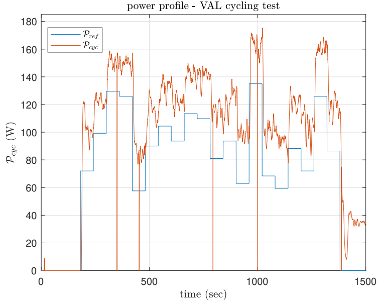
Figure 3.8: Power profile for the validation cycling test (VAL). This test is constituted of steps of random intensity aiming at reproducing an outdoor cycling session. The total duration of this test is 20 min .
