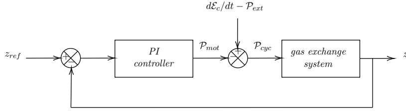
Figure 5.1: Implementation scheme of the PI controller.
