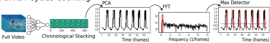
Figure 5.2 – The periodicity counting framework. In Part 1, a Convolutional Neural Network (CNN) is first trained in an unsupervised fashion on the test data, as described in section 5.3.1. Then, it is used to extract an embedding for each image of a video. (1a) shows an example of the 2D PCA projection of these embeddings. The last 50 embeddings are linked chronologically (in red), revealing the cyclic path. (1b) shows the input images whose embeddings correspond to the highlighted points. They belong to different swimming cycles but correspond to the same phase, therefore the points are close in the latent space. In Part 2, we chronologically stack the embeddings obtained from the trained network to form a multi-variate time signal. The PCA’s first component of the signal reduces it into a uni-variate signal. Finally, our Max Detector algorithm is used to count the cycles on the signal, which corresponds to the number of cycles on the video.
