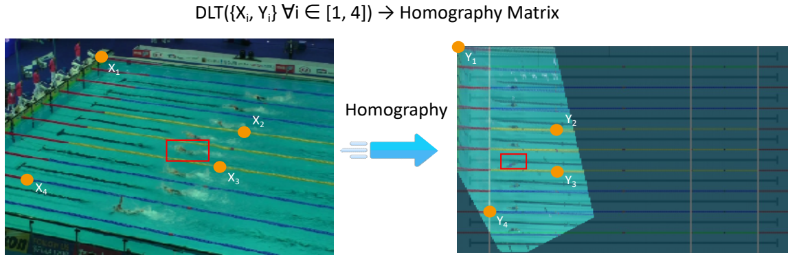
Figure 4.2 – An illustration of the registration. The Dynamic Linear Transform (DLT) operation uses known matches of positions ( X_i with Y_i ) to compute the homography matrix. This matrix can then be used to match a position from one coordinate system to the other. Therefore, the bounding box from the image can be positioned in the pool with this method.
