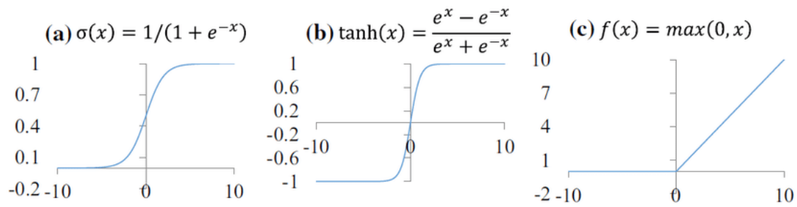
Figure 2.9 – Sigmoid (left), hyperbolic tangent ( tanh ) (center) and Rectified Linear Unit ( ReLU ) (rights) activation functions. The two firsts saturate when moving away from the origin, thus resulting in a weak gradient as their absolute value gets bigger. ReLU has a higher derivative for any positive value, enabling a better gradient back-propagation. Scheme extracted from [54].
