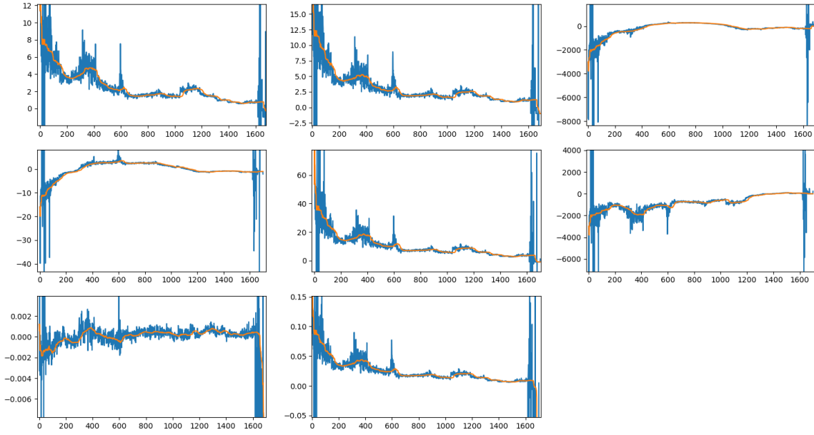
Figure 4.5 – Smoothing of the 8 parameters of the homography matrix estimated for a race (the parameter at position (3,3) is always equal 1). The values are represented through time. The outliers being orders of magnitude different from the truth, they have been cut out in the figure’s frame. Blue: the original signal. Orange: the smoothed signal.
