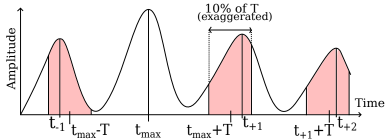
Figure 5.5 – Illustration of Max Detector . Starting from the global maximum’s index t_{max} , the algorithm shifts by one period T and finds the maximum’s index t_{+1} in a window of 10\% of T (in red, exaggerated for a better understanding). This window makes Max Detector robust to period variations. Starting from t_{+1} , this is repeated to find t_{+2} , t_{+3} and so on until reaching the signal’s end. A first iteration goes from t_{max} to the end of the signal and a second from t_{max} to t = 0 .
