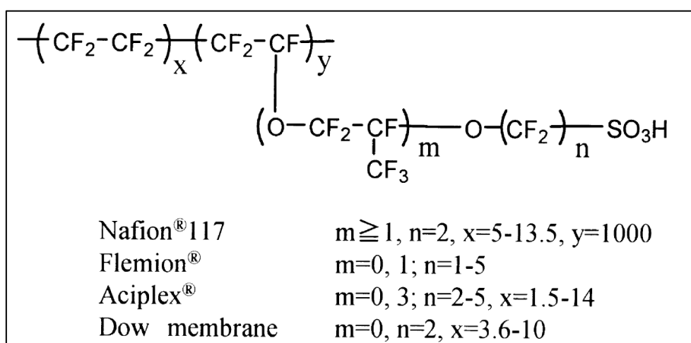
Figure 9: Chemical structures of perfluorinated polymer electrolyte membranes [75].
