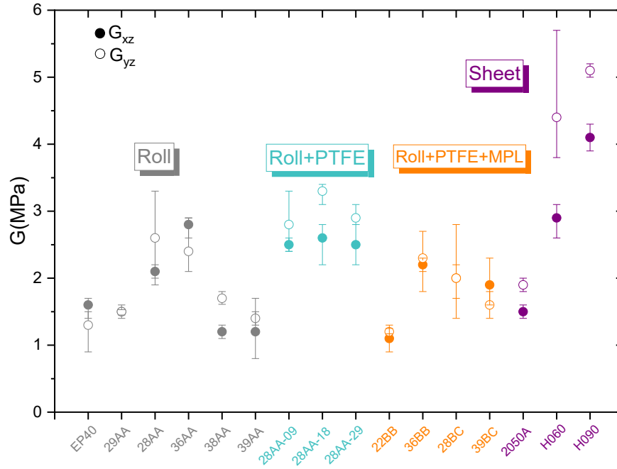
Figure 6: Out-of-plane shear moduli for the different GDL references.
