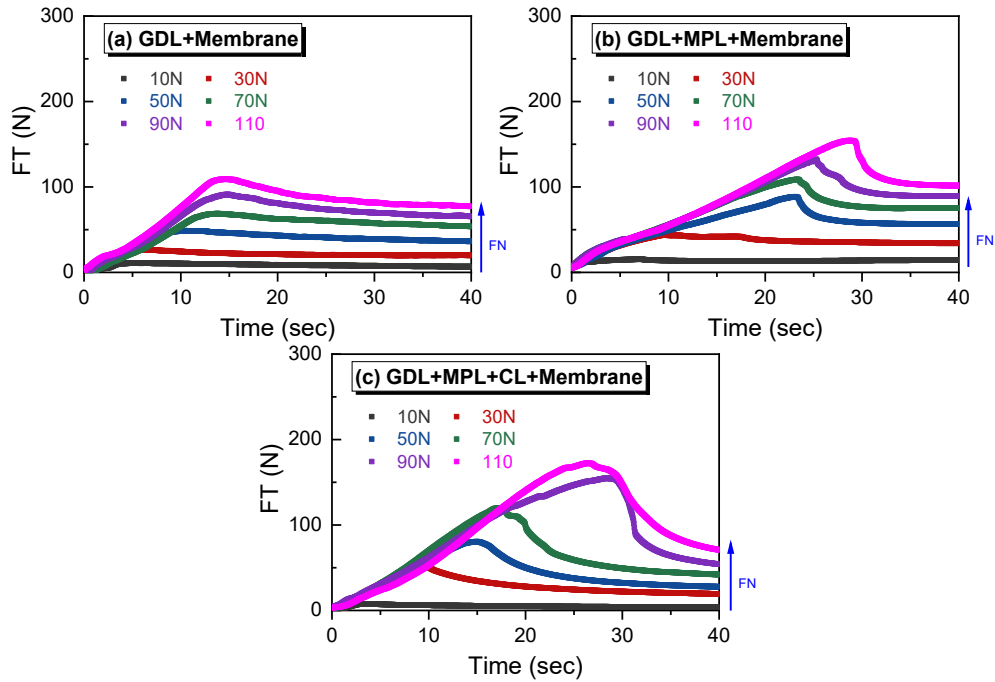
Figure 5: Friction curves for the MEA different configurations (a) GDL+Membrane, (b) GDL+MPL+Membrane, and (c) GDL+MPL+CL+Membrane.
