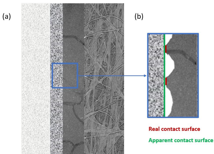
Figure 4: (a) 1/2 MEA layers and (b) difference between apparent and real contact surfaces.
