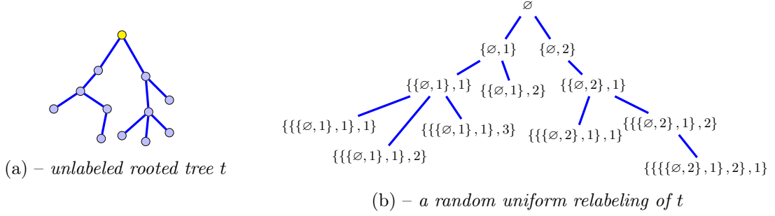
Figure 6.3 – A rooted tree t \in \mathcal{Y}_d with n = 4 (the root is highlighted in yellow).
