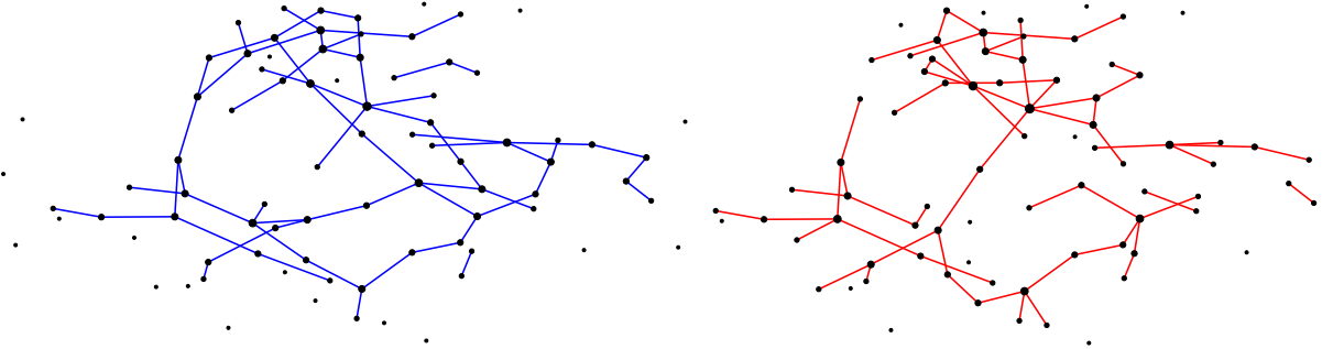
Figure 1.11 – Two samples from \mathbb{G}(n, q, s) with n = 80 , p = 1.9/n and s = 0.8 .
