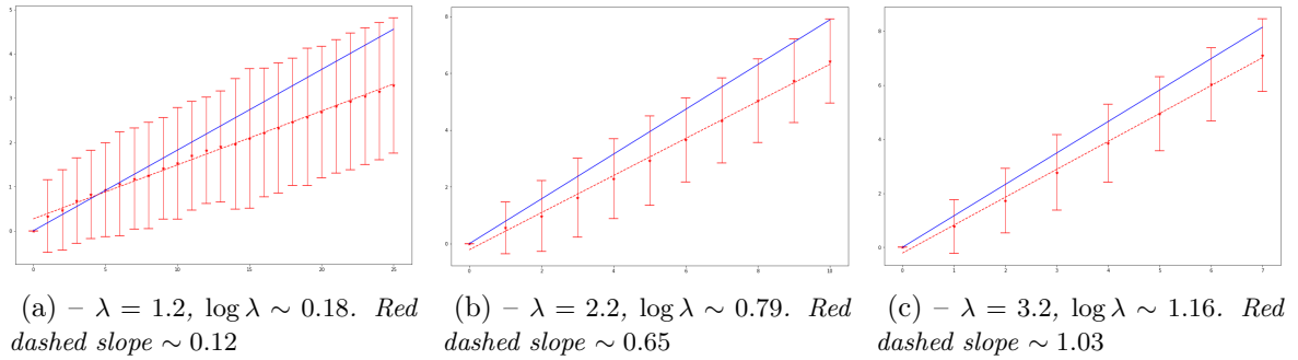
Figure 5.5 – Comparison of d \log \lambda (blue) and \log \mathcal{W}_d(T, T') (red) for \mathcal{W}_d(T, T') \sim \mathbb{P}_d^{(\lambda)} conditioned to survive (100 iterations)
