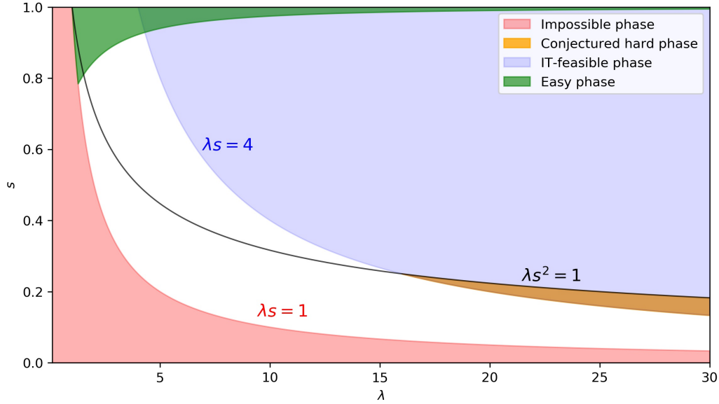
Figure 6.2 – Diagram of the (\lambda, s) regions where partial recovery is known 2 to be IT-impossible ([GML21b]), IT-feasible ([WXY21]), or easy ([GM20] and this chapter). In the orange region, though partial graph alignment is IT-feasible, one-sided detectability is impossible in the tree correlation detection problem, and partial graph alignment is conjectured to be hard (this chapter).
