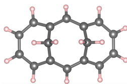
Figure 2.13: Representation of the molecule syn -1,6,8,13-bismethano-[14]-annulene ( C_{16}H_{14} )
