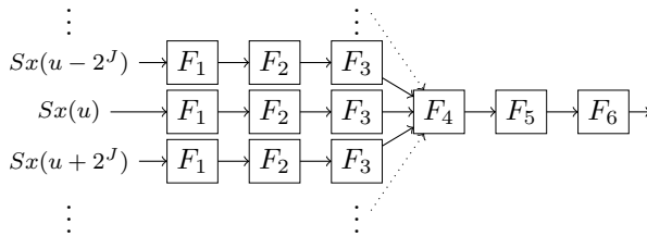
Figure 4.3.1: Architecture of the SLE, which is a cascade of 3 \times 1 convolutions followed by 3 fully connected layers. The ReLU non-linearities are included inside the F_i blocks for clarity.
