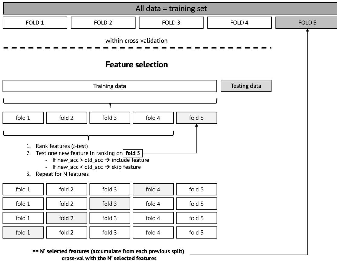
FIGURE 4.4: Feature selection algorithm. Within a cross-validation framework ( CV_{orig} ), this approach uses a nested 5-fold cross-validated SVM ( CV_{nested} ) on a sub-training set (80% of the CV_{orig} training) (Dominguez, 2009), to obtain a subset of selected features, N' = 10 . For each CV_{nested} iteration, features are ranked according to their discriminant power between classes ( t -test). In a forward sequential order, a feature is going to be retained and accumulated in the selected set, if its accuracy is higher than the previous set. The output of this CV_{nested} is a group of 10 selected features on which the CV_{orig} validation set (FOLD 5) is going to be tested. This is repeated for each iteration in CV_{orig} .
