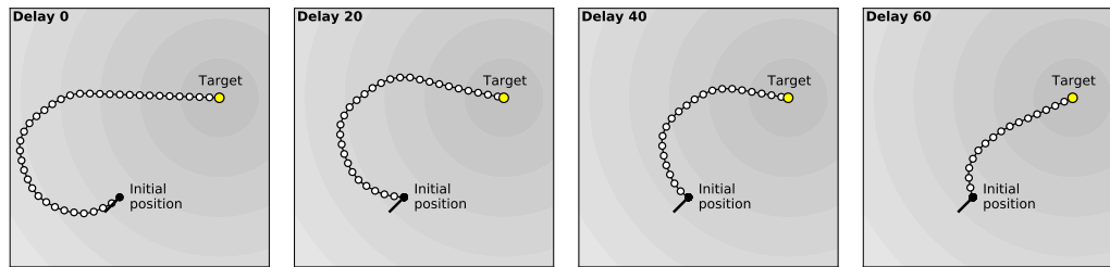
Figure 3.14: Momentum guided reinforcement learning can be understood using an analogy of velocity and acceleration. In this illustration, velocity corresponds to Hebbian learning, which represents the momentum of the trajectory, while acceleration corresponds to reinforcement learning and can modify the velocity vector up to a certain degree (10% in the figure). The illustration simulates the trajectory from a fixed initial position to a target, when the direction of the velocity is continually modified by the acceleration. In the figure, four trajectories with increasing initial delays (left to right) are shown. These delays correspond to the moment when velocity is activated/allowed to initiate the trajectory. Before that, the acceleration influences the direction of the velocity, however without any displacement. When there's no delay, the initial velocity vector can potentially drive the trajectory away from the target (as shown in this specific example), while with longer delays, the acceleration can explore and identify a more conducive direction in order to exhibit a more direct trajectory to the target.
