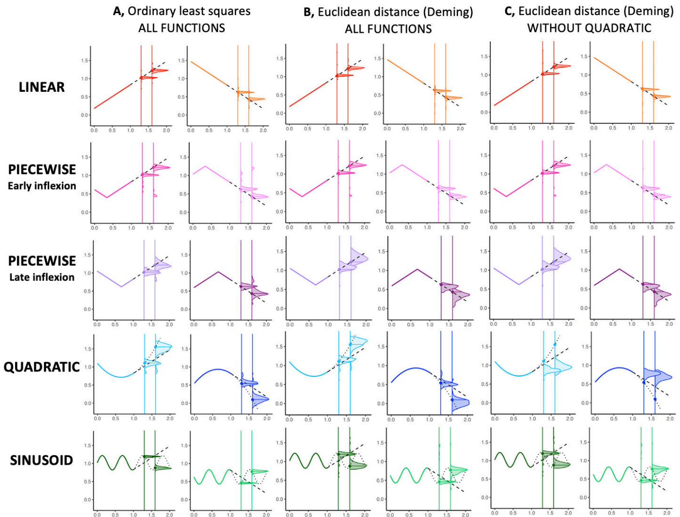
Figure 34. Predictions of three different models. A: Bayesian ideal-observer with full knowledge of the set of functions used, and using ordinary least squares (as appropriate given how the graphs are generated). B: Same as the ideal observer, but using Deming-like minimization of the Euclidean distance of each data point to the regression curve. C: Same as B, but after removal of the quadratic functions from the hypothesis set.
