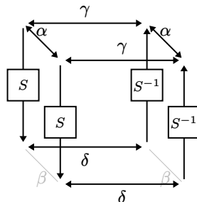
(h) Transition representing a LBCT. This transition requires to know \alpha, \gamma and \delta parameters.
