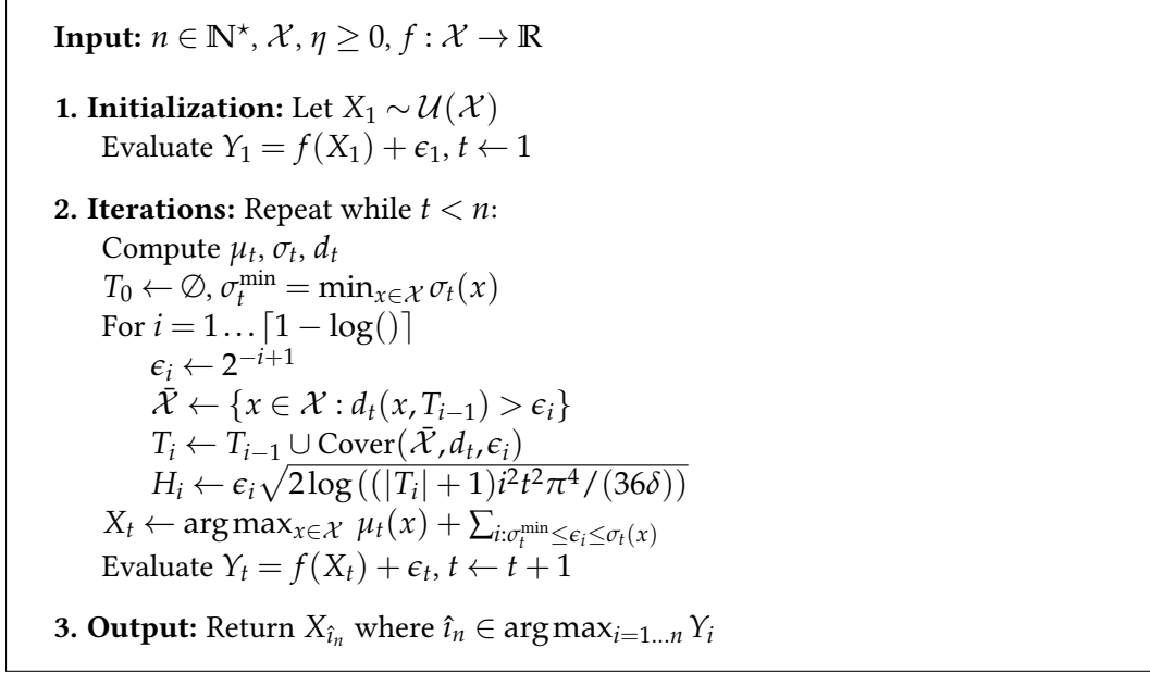
Figure C.1: The Chaining-UCB algorithm
