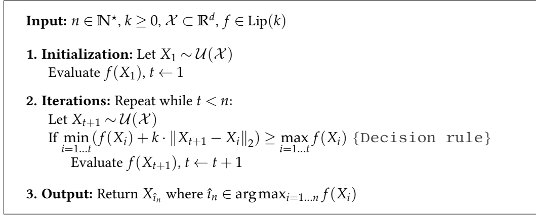
Figure 2.1: The LIPO algorithm
