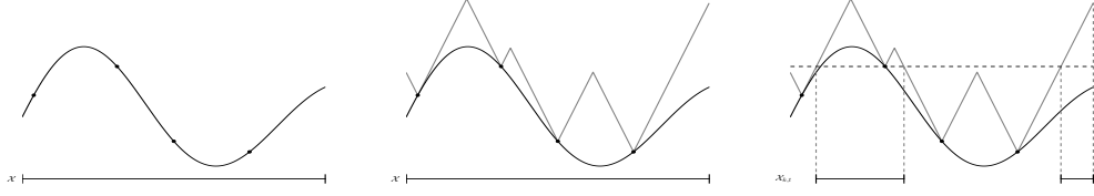
Figure 2.2: Left: A Lipschitz function and a sample of t = 4 evaluations. Middle: In grey, the upper bound UB : x \mapsto \min_{i=1\dots t} f(X_i) + k \cdot \|x - X_i\|_2 . Right: the set of points \mathcal{X}_{k,t} := \{x \in \mathcal{X} : UB(x) \geq \max_{i=1\dots t} f(X_i)\} which satisfy the decision rule.
