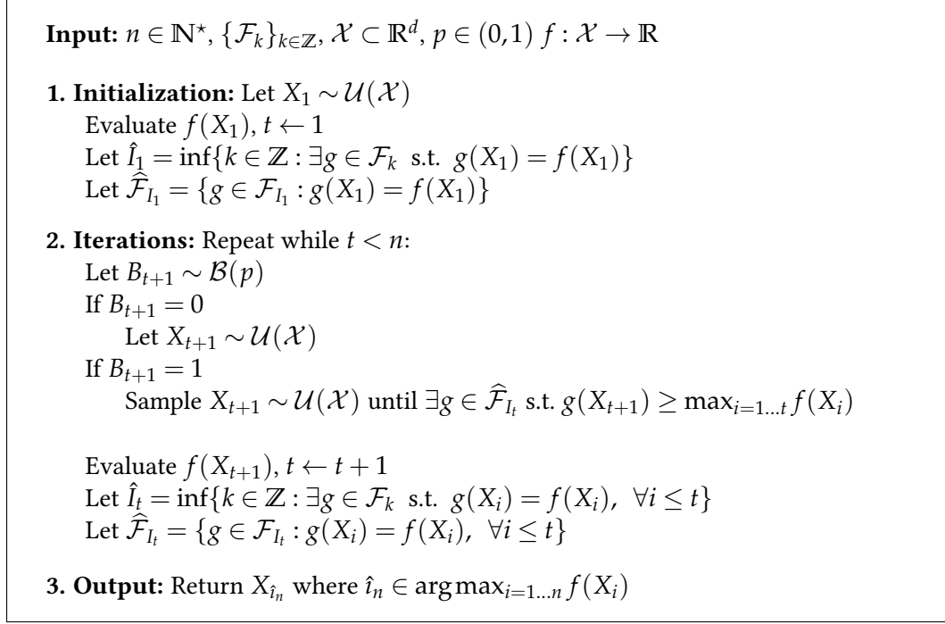
Figure 1.5: Adaptive algorithm over the nested sequence \mathcal{F}_k
