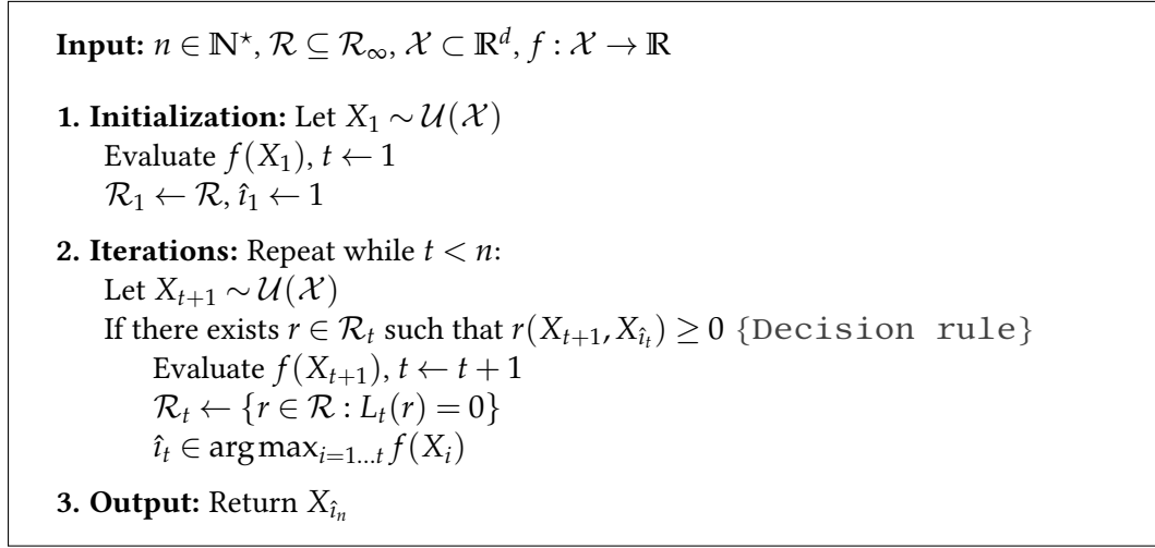
Figure 3.3: The RankOpt algorithm
