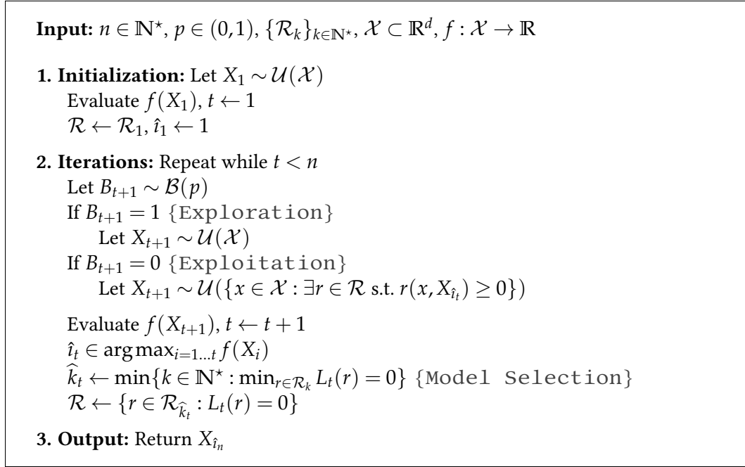
Figure 3.4: The AdaRankOpt algorithm
