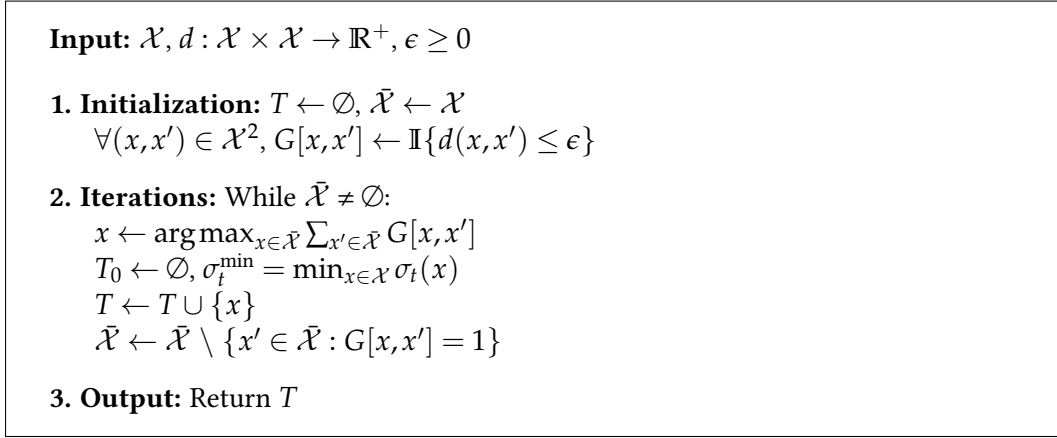
Figure C.2: The Greedy-cover algorithm
