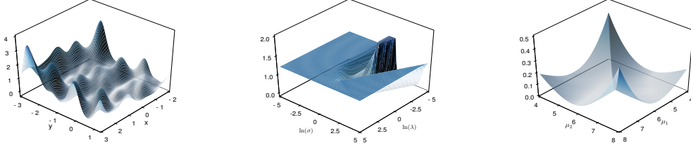
Figure 1.1: Left : Objective function of Example 1.2. Middle : Test function of Example 1.3 computed with the Abalone dataset taken from the UCI machine learning repository. Right : Objective function of Example 1.5 computed with the Iris dataset taken from the UCI machine learning repository.
