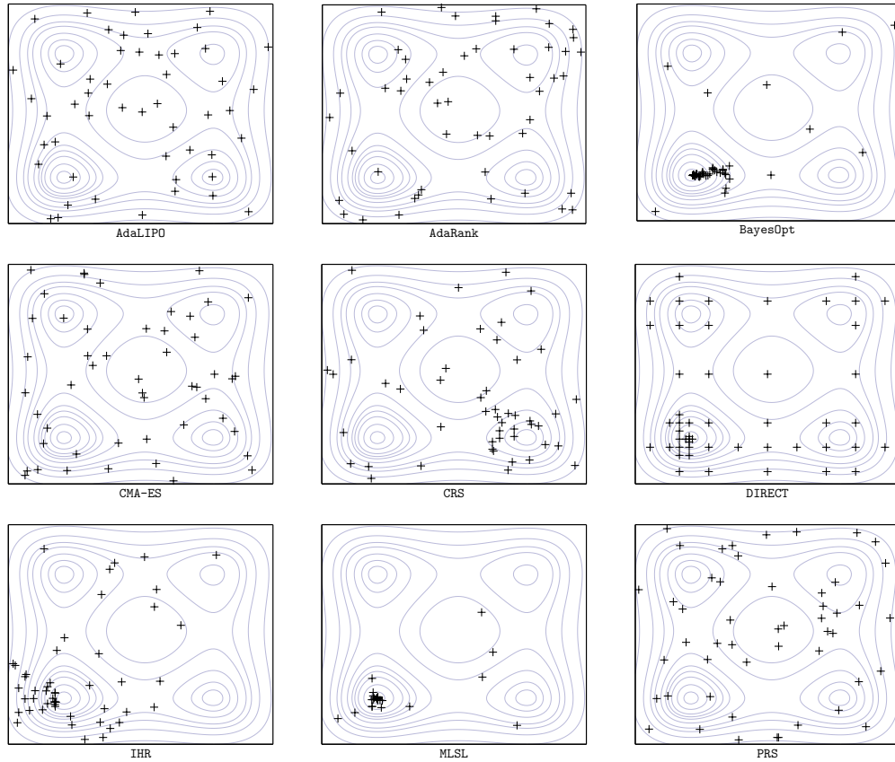
Figure 4.1: Series of n = 50 evaluations points generated by each algorithm on the two-dimensional Styblinski function. The input space \mathcal{X} is set to [-5,5] \times [-5,5] and the optimum of the function is located on the bottom left corner.
