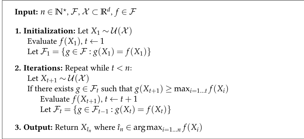
Figure 1.4: Optimization of an unknown function f in the class \mathcal{F}
