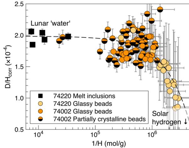
Figure 7.1.3. Hydrogen isotope ratios – corrected for the cosmogenic contribution using a P_D value of (2.17 \pm 0.11) \times 10^{-12} \text{ mol(g rock)}^{-1}\text{Ma}^{-1} – as a function of the inverse of the hydrogen concentration in Apollo 17 high-Ti ('orange') volcanic glass beads (74220; Saal et al., 2013, 74002; Füre et al., 2014) and olivine-hosted melt inclusions (Saal et al., 2013). From Füre et al. (2017).
