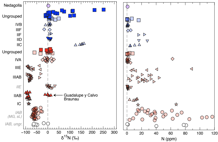
Figure 6.3.1. N isotopic ratios (left) and abundances (right) of iron meteorites (IAB and IIE irons being 'non-magmatic'). NC- and CC-type irons are shown in red and blue, respectively. Data sources: Franchi et al., 1993; Mathew et al., 2000; Murty et al., 2019; Pepin and Becker, 1982; Ponganis and Marti, 2007; Prombo and Clayton, 1993; Sugiura, 1998; Sugiura et al., 2000a. N isotopic compositions of ungrouped, IIAB, and IID irons measured by Füri et al. ( in prep. ) are shown in darker colors; associated N abundances could not be determined because the 20-year-old \text{CO}_2 laser did not permit the quantitative extraction of N from the metal fragments.
