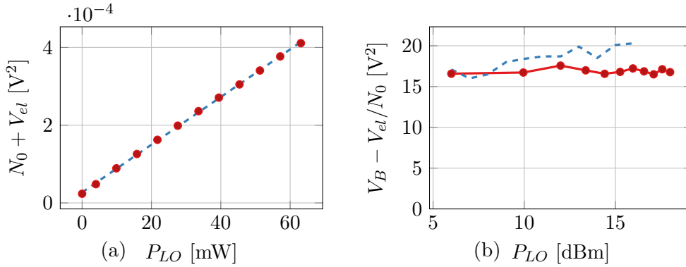
Figure 4.14: (a) Estimation of N_0 + V_{el} [V 2 ] and linear regression (dashed line) vs P_{LO} [mW] and (b) Estimation of V_B - V_{el}/N_0 as a function of P_{LO} , for receiver ② (solid line) and receiver ① (dashed line), performed by integrating the periodogram of the signal over the signal band. We observe that receiver ② has a behavior corresponding to theory while receiver ① does not.
