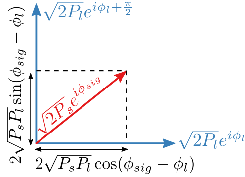
Figure 3.10: Compared to Figure 3.8, the introduction of a secondary LO with a 90^\circ phase shift allows to fully recover the modulated phase of the signal.
