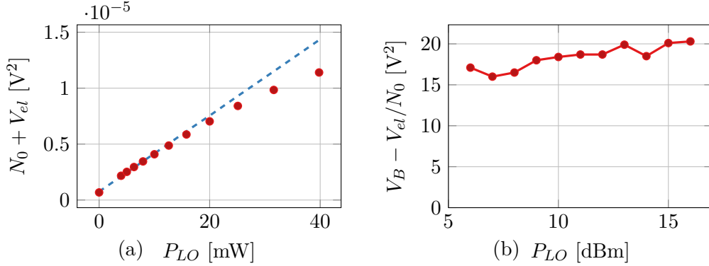
Figure 4.13: (a) Estimation of N_0 + V_{el} [ \text{V}^2 ] and linear regression (dashed line) vs P_{LO} [mW] and (b) estimation of V_B - V_{el}/N_0 as a function of P_{LO} , for receiver ①, performed by integrating the periodogram of the signal over the signal band. We observe that it is not constant with P_{LO} , not conforming to theory.
