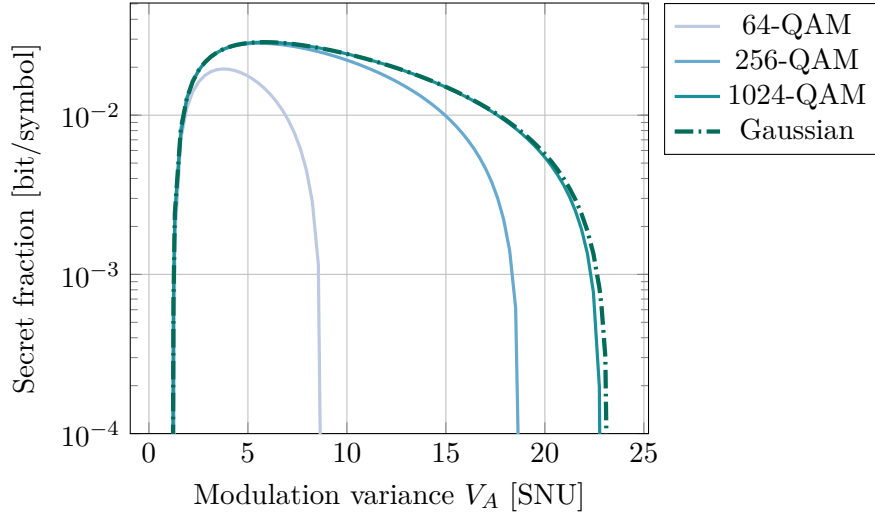
Figure 2.5: Secret fraction [bit/symbol] vs modulation variance V_A [SNU] for a Gaussian channel with transmittance T = -5 dB, corresponding to 25 km of single mode fiber, and excess noise variance \xi_B = 0.01 SNU, trusted receiver with quantum efficiency \eta = 0.65 and electronic noise variance V_{el} = 0.1 SNU, and reconciliation efficiency \beta = 0.95 .
