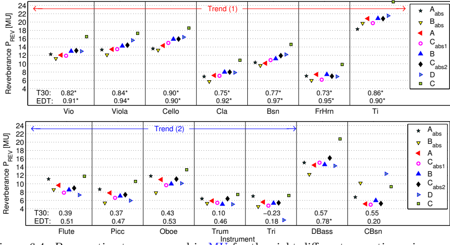
Figure 6.4: P_{REV} estimates expressed in MU for the eight different acoustic environments. For each instrument the correlation between P_{REV} and T_{30} and EDT is shown. Values marked with asterisks indicate that the corresponding P_{REV} estimate is linearly related with T_{30} and/or EDT ( p < 0.05 ).
