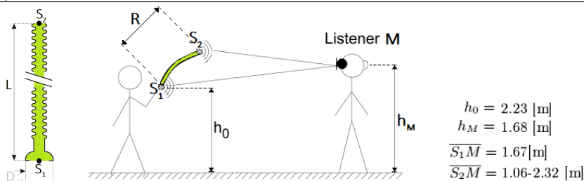
Figure 2.2: Schematic drawing of a hummer. The hummer has a length L of 70 cm, the inlet ( S_1 ) has an entrance diameter D_{\text{ent}} of 3.3 cm. The opposite end of the hummer is identified as the outlet ( S_2 ). Note that the distances in this drawing are not to scale. Some pictures of the hummer can be found in the study by Hirschberg et al. (2013) . This figure was adapted from Nakiboğlu et al. (2012) .
