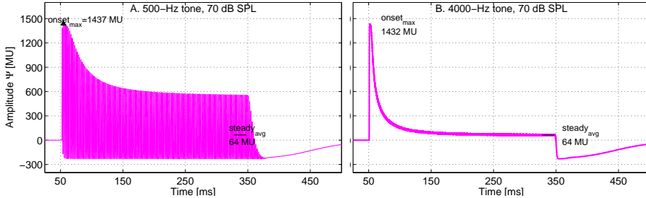
Figure C.9: Output of the adaptation loops for the same two sine tones used in Figure C.5 but for an overshoot limitation of 10. The onset and steady-state amplitudes are 1437 and 64 MU for the 500-Hz tone and 1432 and 64 MU for the 4000-Hz tone, respectively.
