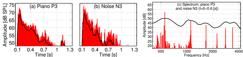
Figure 3.3: (a) Waveform of the piano P3 converted to SPL, and (b) one realisation of its resulting ICRA noise at an SNR= 0 dB. The thick black lines correspond to the Hilbert envelope of the waveforms. (c) Spectra of the piano sound (red) and the ICRA noise (black thick line) averaged over the first 0.6 s of both waveforms.
