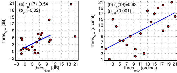
Figure 4.7: Regression analysis between the experimental \text{thres}_{\text{exp}} and simulated \text{thres}_{\text{sim}} as: (a) SNR thresholds, and (b) ordinal thresholds. The linear regression of panel (a) is related to the Pearson correlation r_p , while the regression of panel (b) to the Spearman correlation r_s . Two pairs of points were removed from the analysis to obtain an r_p(17) = 0.54 , p = 0.02 , due to the lack of \text{thres}_{\text{exp}} values above 12 dB. A Spearman correlation of r_s(19) = 0.63 , p < 0.001 was obtained.
