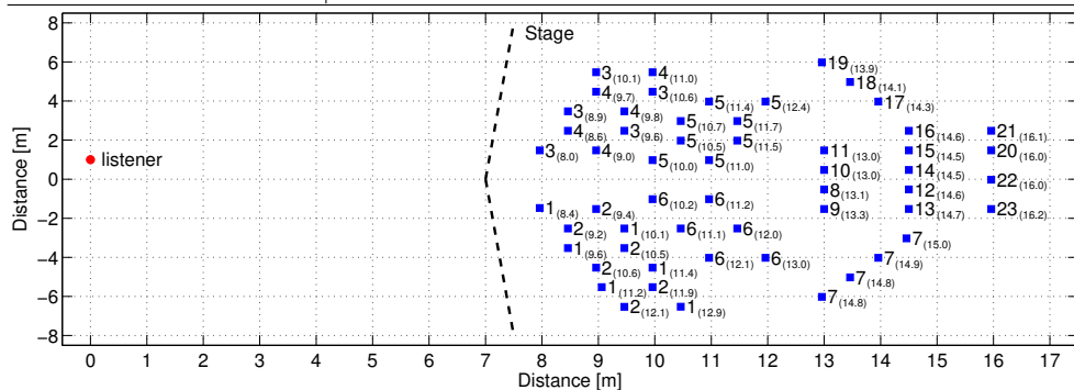
Figure 6.3: Distribution of the orchestra as used in Odeon for room D. The distances along the abscissa are referenced to the position of the virtual listener. The listener is located 7 m in front of the stage and 8 m far away from the closest “musician”. This position is located in the audience area already which is further extended behind the listener (it would correspond to negative distances in this figure, not shown). The musicians are indicated by numbers between 1 and 23* (see Table 6.3 for the corresponding labels). The numbers between brackets represent the (Euclidean) distance in m from each musician to the listener.
