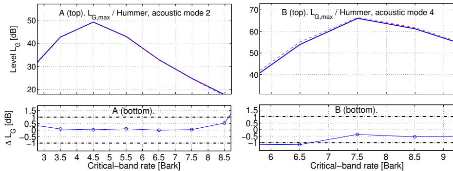
Figure 2.5: Maximum critical-band levels L_{G,\max} for recorded (blue solid line) and synthesised (red dashed line) hummer signals in the acoustic modes 2 (panel A) and 4 (panel B). In the bottom panels, the differences between the recorded and synthesised signals are shown. The black dashed-dotted lines indicate the assumed JND of 1 dB.
