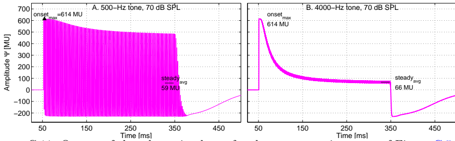
Figure C.11: Output of the adaptation loops for the same two sine tones of Figure C.5 but for an overshoot limitation of 5. The onset and steady-stage amplitudes are 614 and 59 MU for the 500-Hz tone and 614 and 66 MU for the 4000-Hz tone, respectively.
