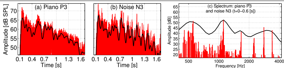
Figure 5.4: (a) Waveform of a reverberant sound of piano P3 converted to SPL, and (b) one realisation of its resulting ICRA noise at an SNR=0 dB. The thick black lines correspond to the envelope of the waveforms. (c) Spectra of the piano sound (red) and the ICRA noise (black thick line) averaged over the first 0.6 s of both waveforms.
