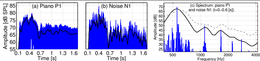
Figure 5.2: (a) Waveform of a reverberant sound of piano P1 converted to SPL, and (b) one realisation of its resulting ICRA noise at an SNR= 0 dB. The thick black lines correspond to the envelope of the waveforms (LPF, f_{\text{cut-off}} = 20 Hz). (c) Spectra of the piano sound (blue) and the ICRA noise (black thick line) averaged over the first 0.6 s of both waveforms. The grey dashed line represents the spectrum of the ICRA noise, using the old version A.
