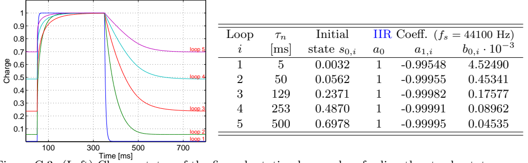
Figure C.3: (Left) Charge status of the five adaptation loops when feeding the steady-state input shown in Figure C.2. The steady signal was preceded by the inner-hair cell processing, so the onset and the offset of the signal were slightly smoothed. (Right) Some parameters that characterise the adaptation loops. The steady-state charge was assessed considering a minimum instantaneous amplitude of lv_{\min} = 1 \cdot 10^{-5} (0 dB SPL) of the input signal.
