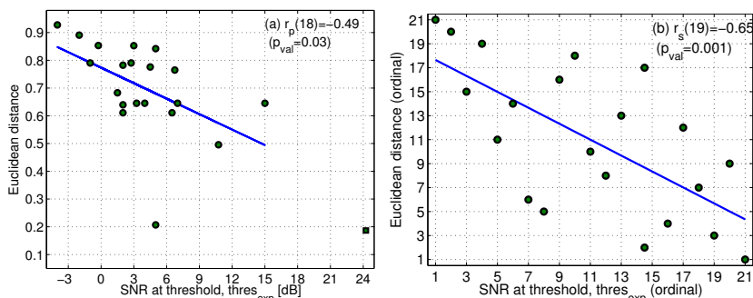
Figure 5.13: Scatter plots and regression analysis between the results of the instrument-in-noise (SNR thresholds, \text{thres}_{\text{exp}} ) and triadic comparisons tests (Euclidean distances). The linear regression of panel (a) is related to the Pearson correlation r_p , while the regression in panel (b) to the Spearman (rank-order) correlation r_s . One pair of points was removed from the analysis to obtain an r_p(18) = -0.49 , p = 0.03 , due to the lack of \text{thres}_{\text{exp}} values above 15 dB. A Spearman correlation of r_s(19) = -0.65 , p = 0.001 .
