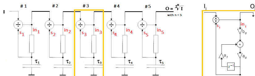
Figure C.1: (Left) Chain of five adaptation loops. (Right) Digital implementation of the adaptation loop i . The labels in_i indicate the input to the adaptation loop i , which in turn represents the input for the divisor of the next element. The input and output of the adaptation loop i are indicated by I_i and O_i . We keep however the notation of in_i (which is equal to I_i ) and s_i ( O_i[n] = in_i[n]/s_i[n-1] ) because the structure between in_i and s_i is an IIR LPF which is characterised by Equation C.2, whose constants are derived from \tau_i .
