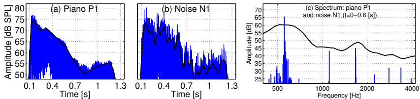
Figure 3.2: (a) Waveform of the Viennese piano P1 converted to SPL, and (b) one realisation of its resulting ICRA noise at an SNR= 0 dB. The thick black lines correspond to the Hilbert envelope of the waveforms (LPF with cut-off at 20 Hz). (c) Spectra of the piano sound (blue) and the ICRA noise (black thick line) averaged over the first 0.6 s of both waveforms.
