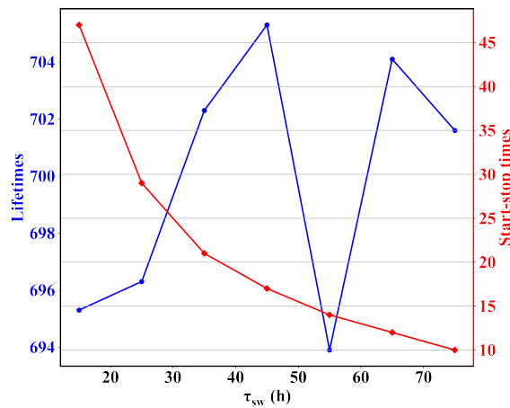
Figure 6.5: Simulated lifetimes and start-stop times under investigated \tau_{sw}
