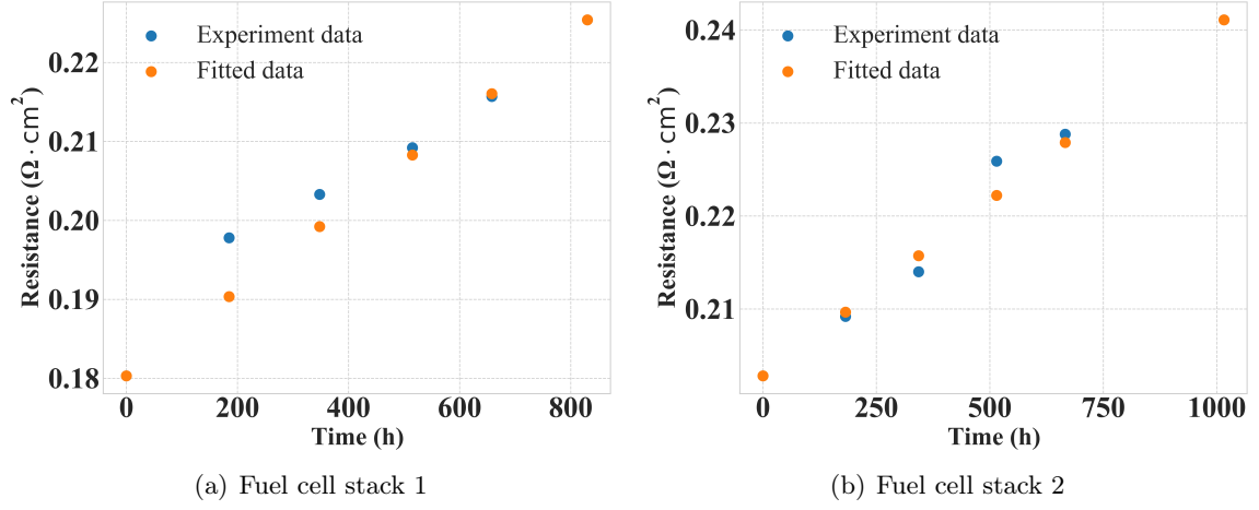
Figure 3.9: Parameter estimation results using MoM method.
