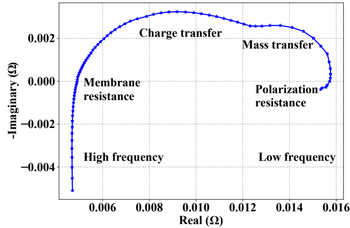
Figure 1.6: Typical Nyquist plots for a fuel cell (EIS spectra).
