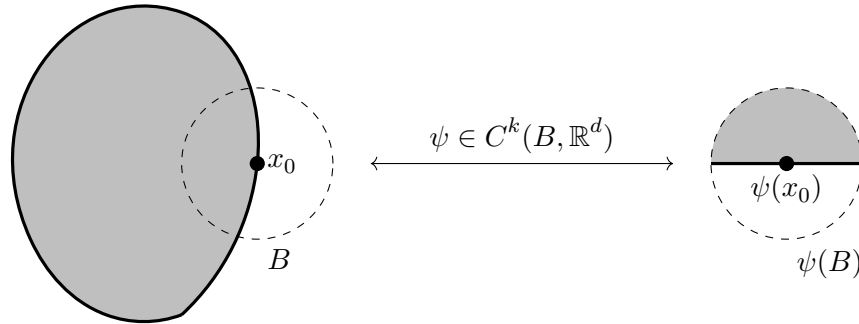
Figure 3.1: Local C^k regularity for a shape. The C^k -diffeomorphism \psi transforms the boundary part \partial\Omega \cap B into a part of the plane of equation x_d = 0 .
