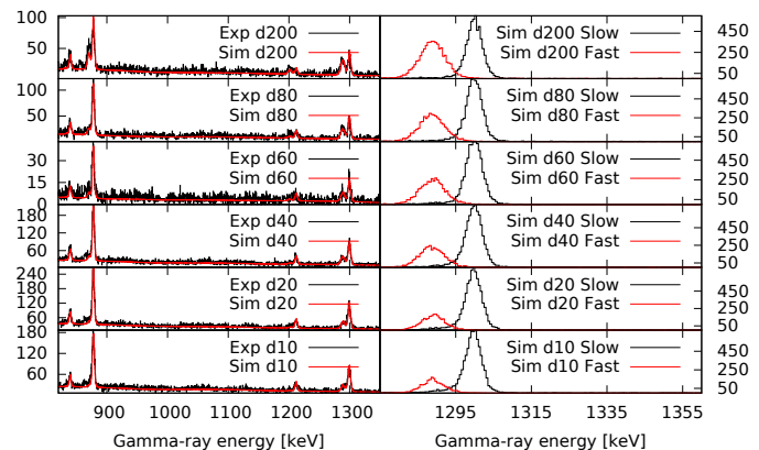
Fig. 6. Realistic simulation of the first AGATA@GANIL experiment. In these simulations the populations and lifetime of levels have been adapted to reproduce experimental spectra as a function of distance between the target and the degrader foil. The purpose of the simulations was to determine the peak shape of the "slow" component.
