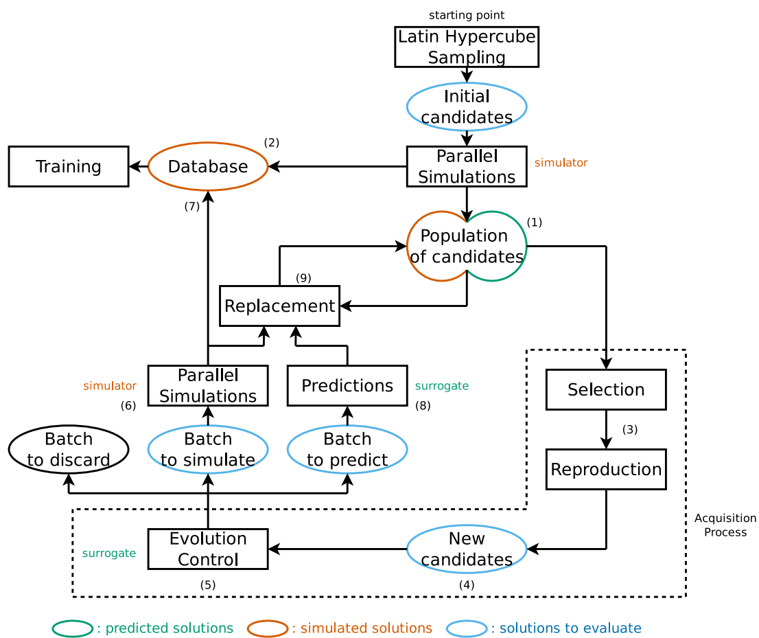
Figure 2.2: SaaEF framework. The ellipses represent the sets of candidate solutions along with their objective values or not, while the rectangles stand for the operators.
