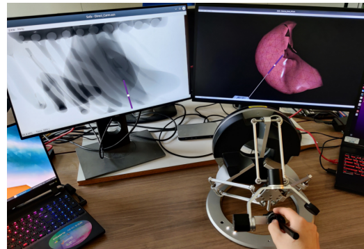
Figure 4.21: Trials setup.
