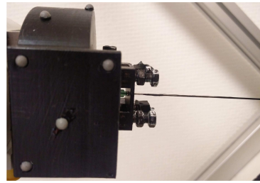
Figure 4.9: Needle support.
