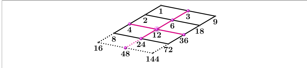
Figure 3.30: n = 144 . A_{CM} = 18\mathbb{I}_2 \oplus 16\mathbb{I}_3 .
