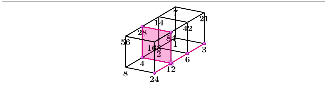
Figure 3.10: n = 168 . A = 42\mathbb{I}_2 \oplus 8\mathbb{I}_3 .
