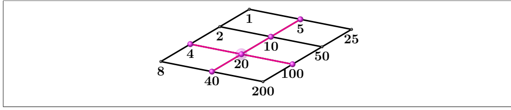
Figure 4.5: n = 200 . A_{CM} = 50\mathbb{I}_2 \oplus 8\mathbb{I}_3 .
