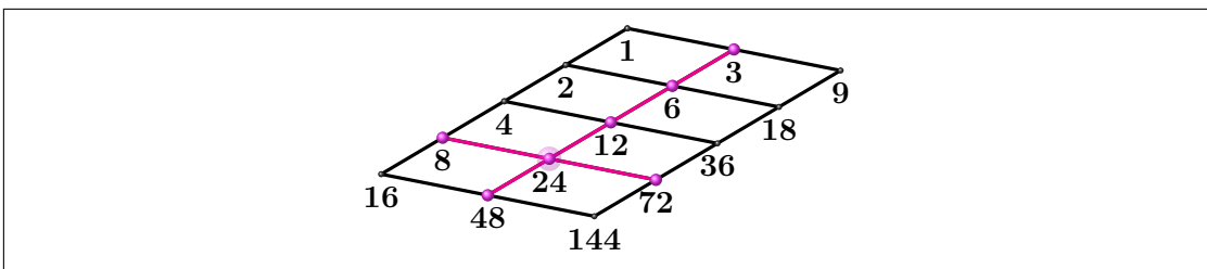
Figure 3.7: n = 144 . A_{CM} = 36\mathbb{I}_2 \oplus 16\mathbb{I}_3 .
