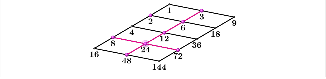
Figure 3.17: n = 144 . A = 16\mathbb{I}_3 \oplus 36\mathbb{I}_2 \oplus \mathbb{I}_2 .
