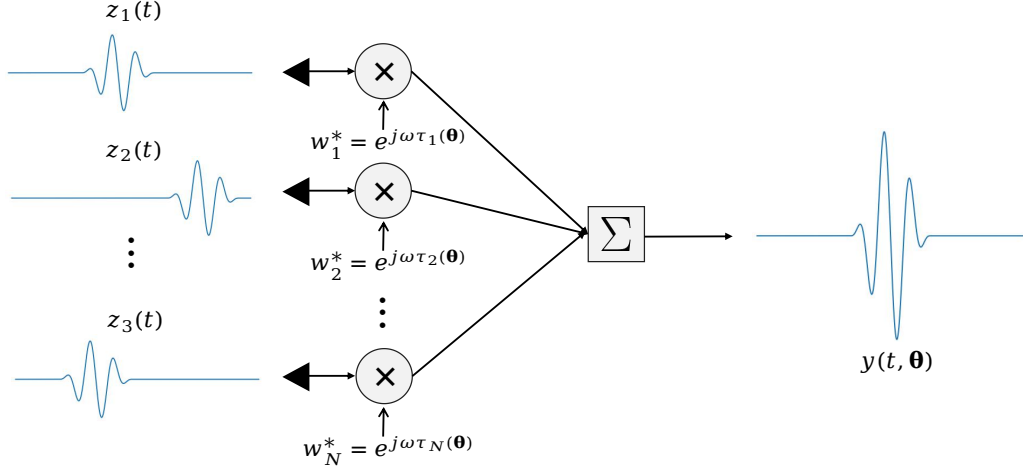
Figure 2.4: Illustration of delay-and-sum beamforming to achieve source localization. The filter weights \mathbf{w}(\theta) apply delays to the input signals based on the distance between each antenna element and candidate position \theta . The beamformer outputs the sum of the delayed signals which presents constructive interference when the candidate \theta matches the true source location.
