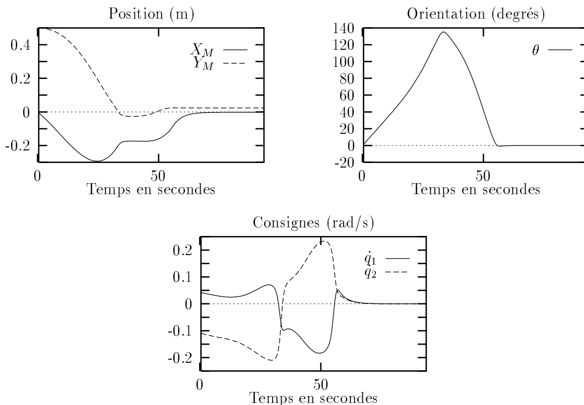
Fig. 6.12: Simulation pour X_M = 0\text{m} , Y_M = 0.5\text{m} , \theta = 0^\circ
