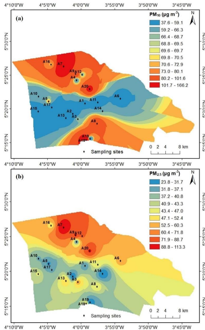
Fig. 6. Spatial variation of PM 10 (a) and PM 2.5 (b) concentrations in Abidjan (Cote d'Ivoire), where black diamonds represent each measurement site.
