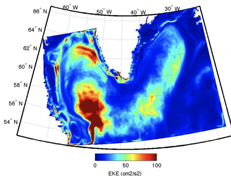
Figure 3.1: Surface eddy kinetic energy in SAKAI configuration for the period 1990-1999.
