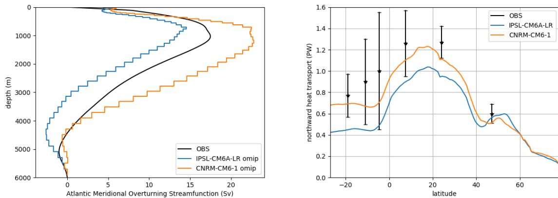
Figure 4.2: MOC streamfunction at 26^{\circ}\text{N} (left) and meridional heat transport in the Atlantic as a function of latitude (right) in IPSL-CM6A-LR (blue) and CNRM-CM6-1 (orange) OMIP simulations (last cycle, ie 1950-2009) and in observations (black, for period 2004-2017). Observations of MOC come from the RAPID project, while observations for the meridional heat transport are taken from Ganachaud and Wunsch (2003).
