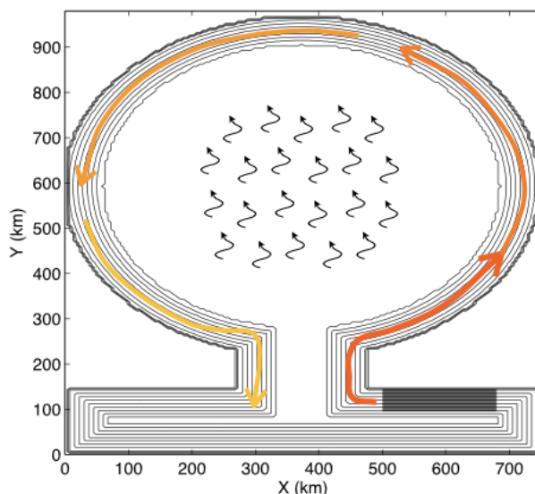
Figure 2.3: Bathymetry of an idealized convective basin (contour interval 100 m, ie the flat area is at 1000m depth), forced by surface buoyancy fluxes in the interior (represented by wiggling arrows) and a barotropic boundary current (applied through restoring in the dark grey shaded area). Coloured arrows represent the circulation of the boundary current around the basin, relatively warm at the inflow and progressively colder as it loses heat due to turbulent exchanges with the interior.
