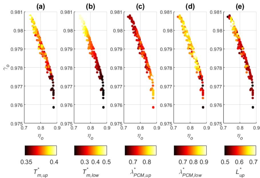
Figure 5.16: Multi-objective optimization results of objectives versus variables for Design A+.
