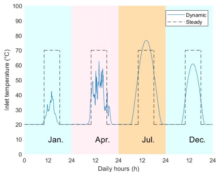
Figure 5.5: Steady and dynamic inlet temperature of thermozone packed-bed tank for four seasonal days.
