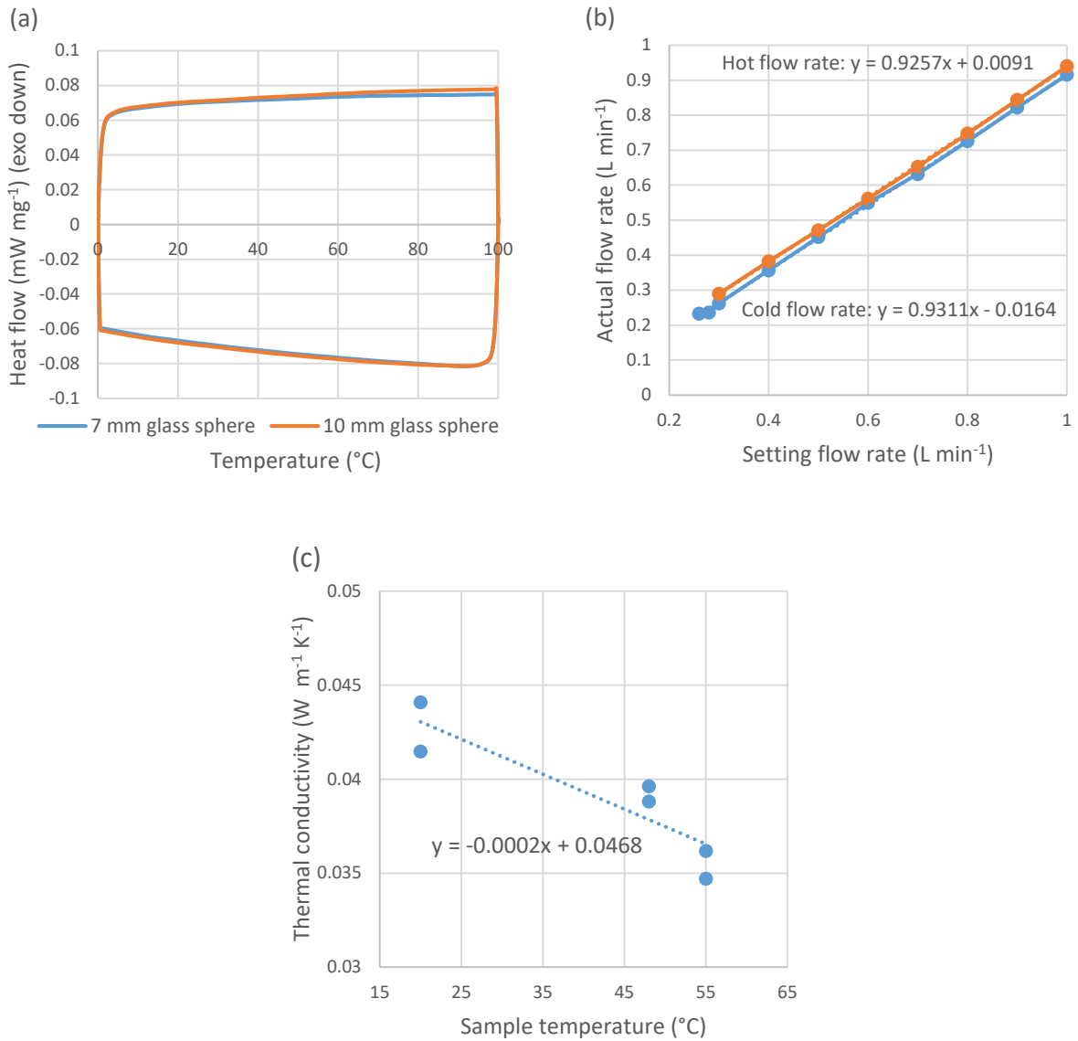
Figure A 4.1: (a) Differential scanning calorimetry curves of glass sphere in range of 0-100 °C; (b) Calibrated flow rates of hot and cold water; (c) Measured thermal conductivity of insulation with temperature increase.
