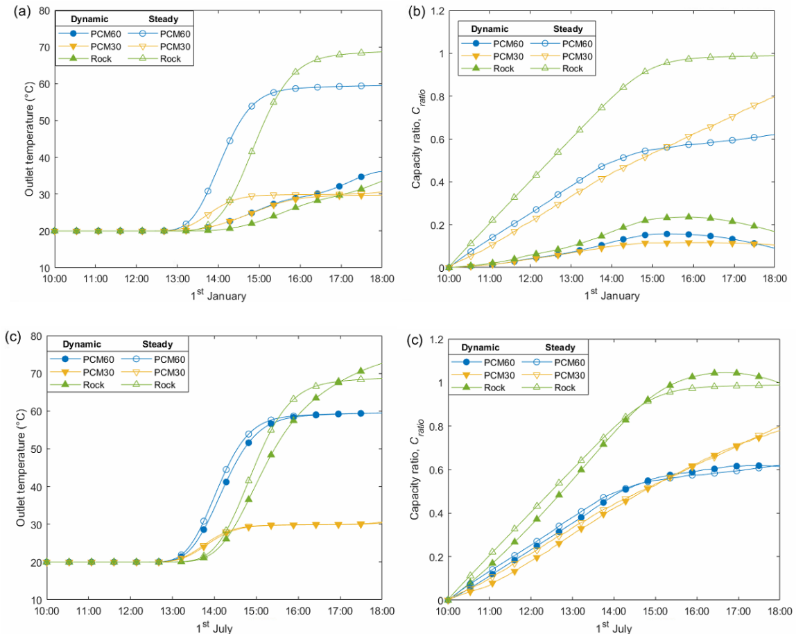
Figure 5.9: Evaluation of steady and dynamic inlet temperature for one representative day in charging (1 st January, 1 st July): (a)(c) outlet temperature profile; (b)(d) capacity ratio. ( N=300 , M=300 , F=10 ).
