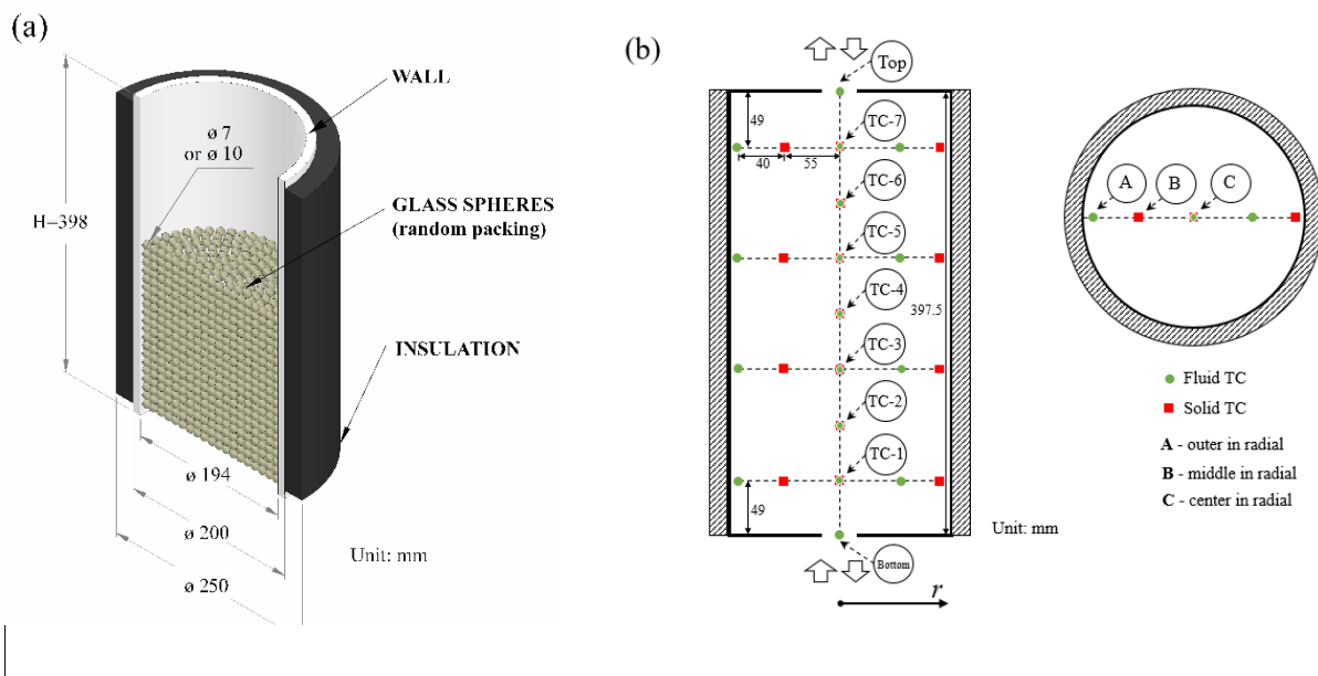
Figure 4.1: Laboratory-scale SHTPB tank tested: (a) Geometry and dimensions; (b) axial and radial thermocouples locations inside the tank.
