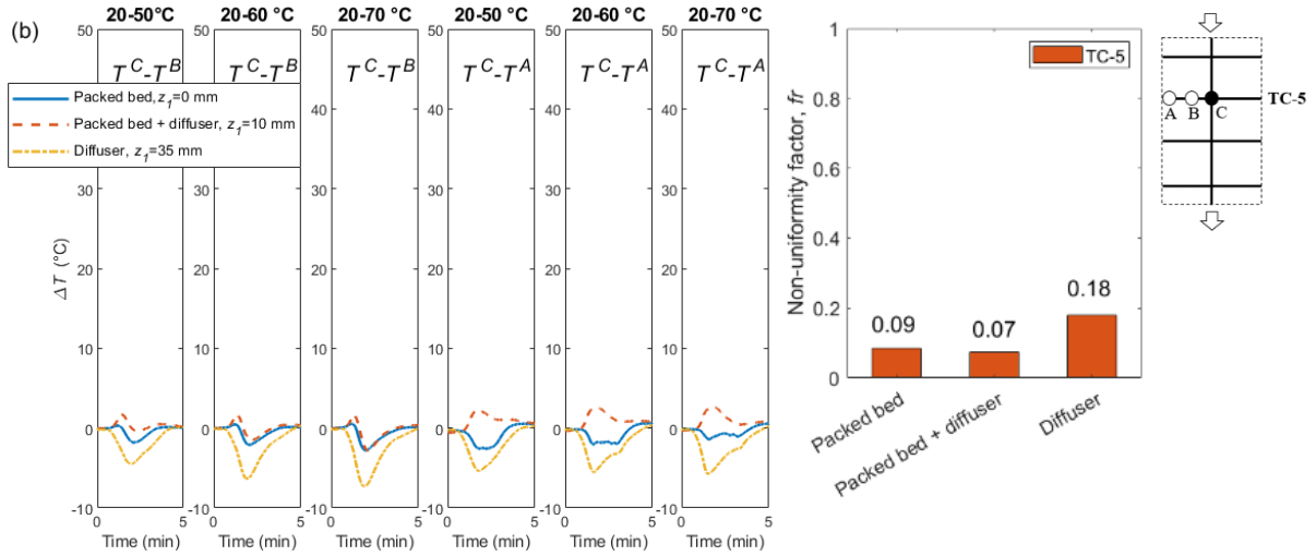
Figure 4.10: Radial temperature difference inside the SHTPB tank with different tested inlet configurations: (a) TC-7 position; (b) TC-5 position (Case 3, 5 & 6: D_p=10 mm; \dot{V}_f=1.5 L min ^{-1} ; charging).
