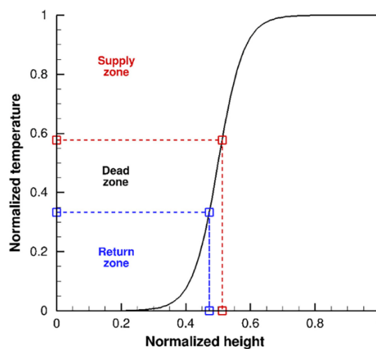
Figure 2.3: Intermediate “dead zone” in conventional rock-filled thermocline tank [36].
