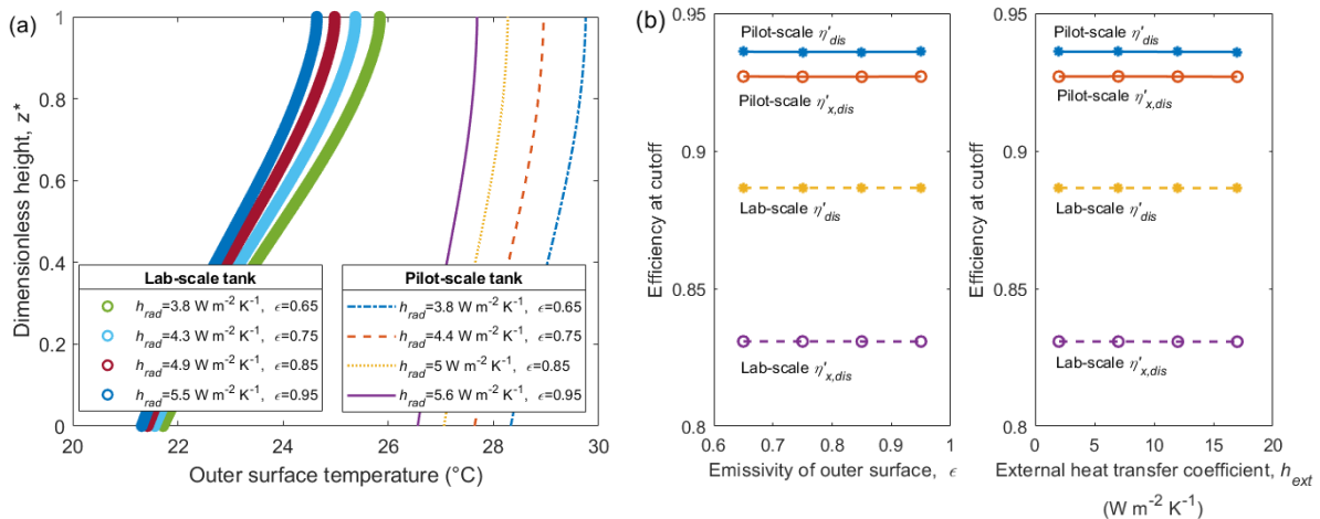
Figure 3.13: (a) Outer surface temperature at cutoff with emissivity variation; (b) energy and exergy efficiency at cutoff with external heat transfer coefficient variation.
