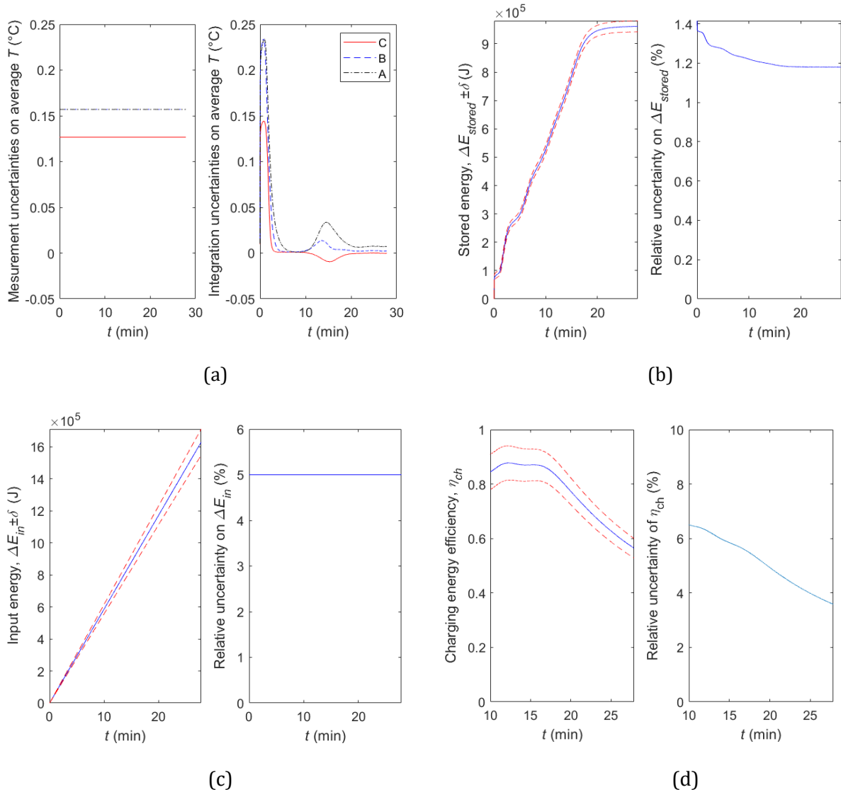
FigureA 4.2: Uncertainty of the validation case: (a) bed average temperature; (b) stored energy ( E_{\text{stored}} ) based on bed average temperature; (c) input energy ( E_{\text{in}} ) based on bed average temperature; (d) charging energy efficiency ( \eta_{\text{ch}} ) based on bed average temperature.
