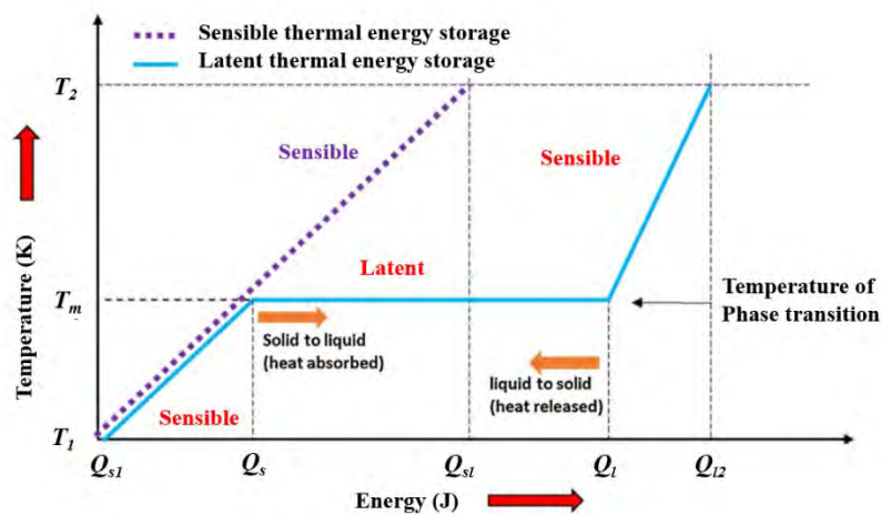
Figure 2.4: Phase change temperature profiles of solid-liquid transition [55][56].
