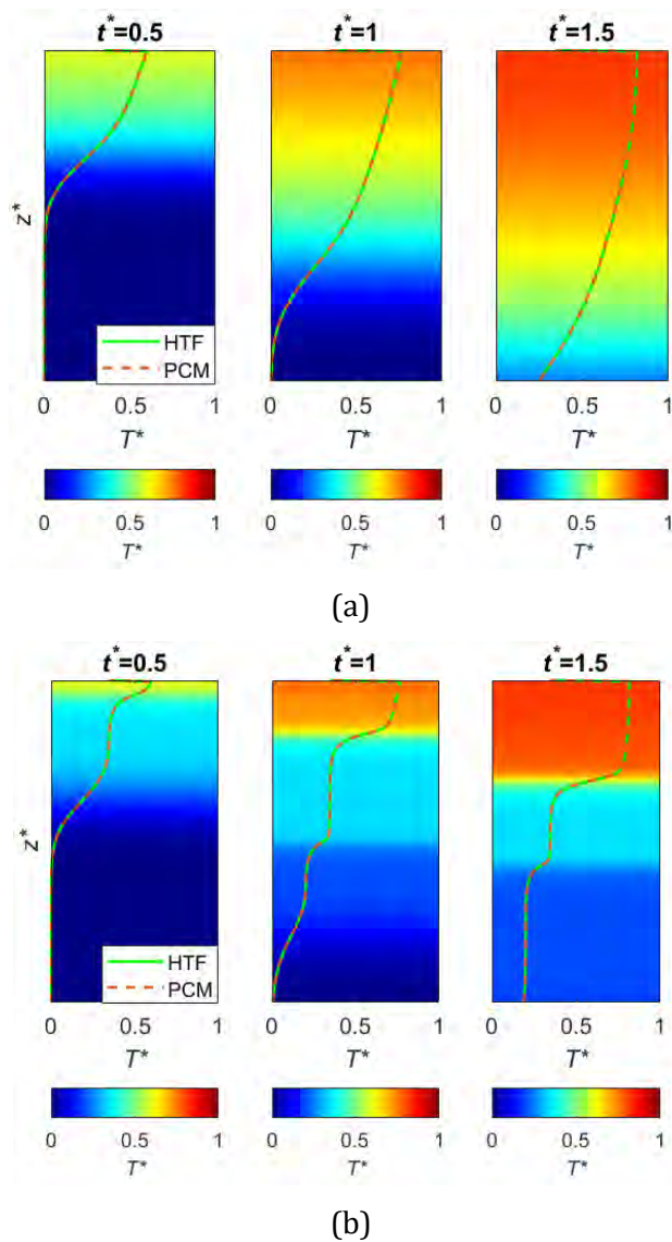
Figure 5.19: Temperature profiles at dynamic inlet condition in greenhouse in 1 st July:
