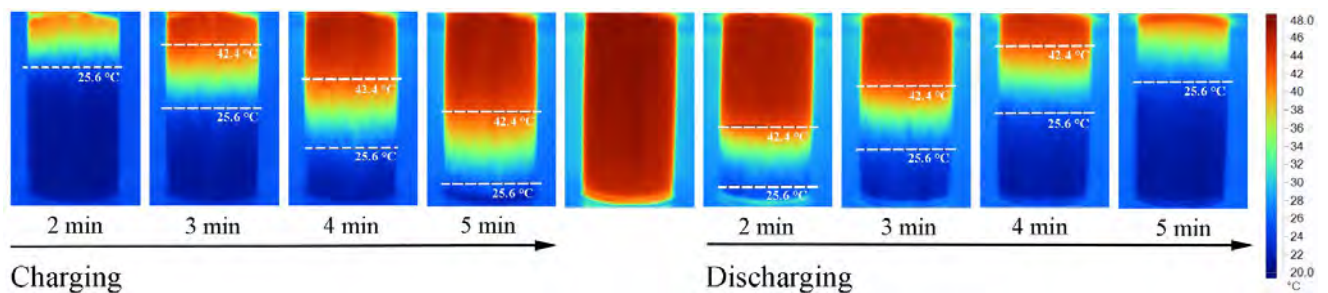
Figure 4.12: Experimental thermal infrared images of charging and discharging process ( T_C/T_H=20/50 °C, D_p=10 mm, 1.5 L min ^{-1} , diffuser z_1=10 mm, no insulation, \epsilon=0.90 , T_{amb}=20.7 °C).
