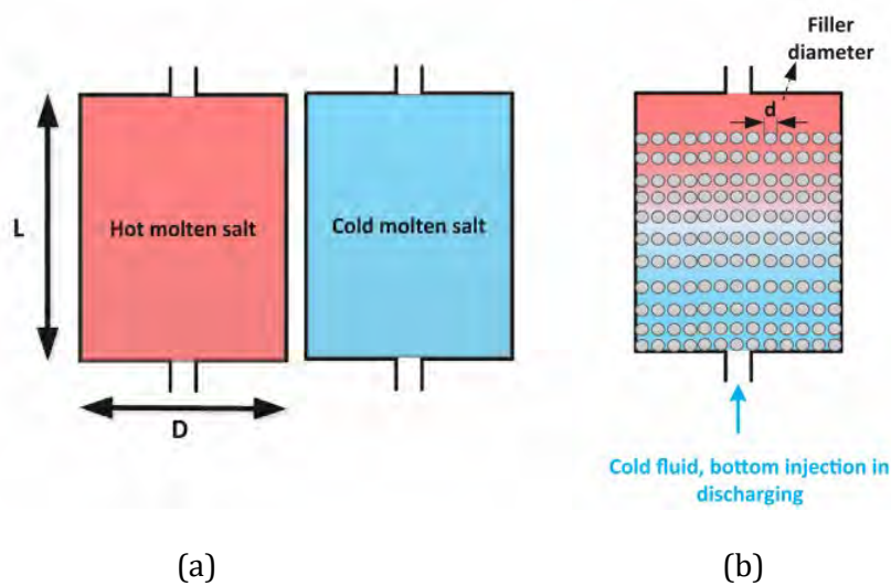
Figure 2.11: Different packing strategies of thermocline systems integrated into a 19.9 MWe Gemasolar CSP: (a) two-tank with specific storage cost of 24.55 US$ kWh th -1 ; (b) dual-media thermocline tank filled concrete with specific storage cost of 9.38 US$ kWh th -1 [70].
