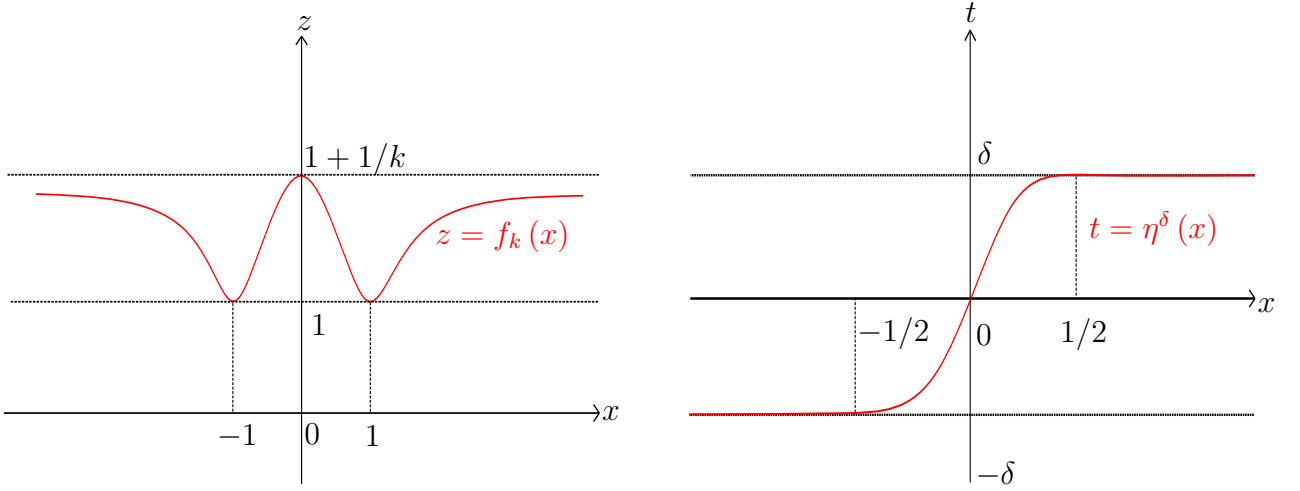
Figure 3.1: Functions f_k (on the left) and \eta^\delta (on the right)
