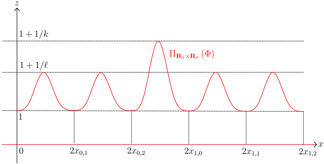
Figure 3.3: Front projection of \Phi when r = 1 and s = 2
