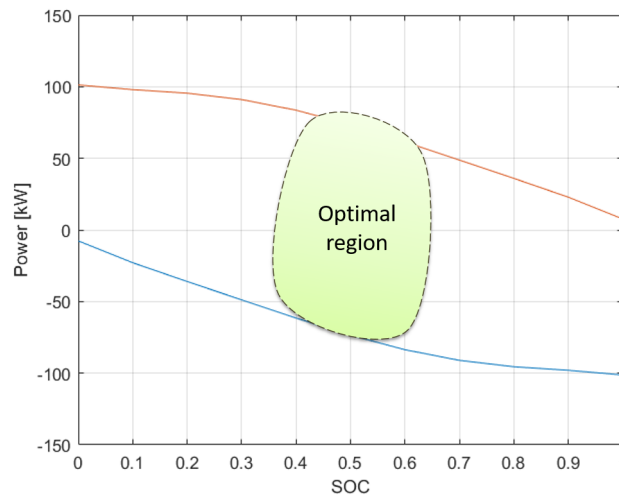
Figure 4.10 – Lithium-ion battery charging and discharging capability depending on the SOC
