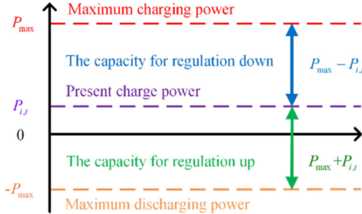
Figure 4.11 – Definition of the capacity for regulation up and regulation down [6]
