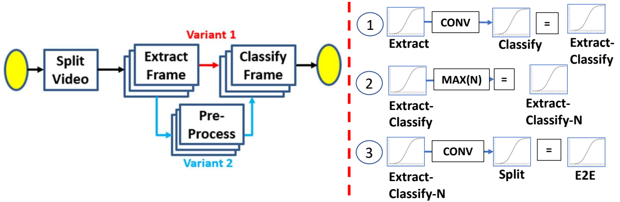
Figure 6.8. Video Analytics DAG. Split function downloads input video and splits it into chunks. Each chunk is passed to an instance of Extract function — extracting a representative frame, sent either to Classify function (Variant #1), or sent to Pre-process function and then Classify (Variant #2). The steps of estimating E2E latency distribution for Variant #1 are on the right.
