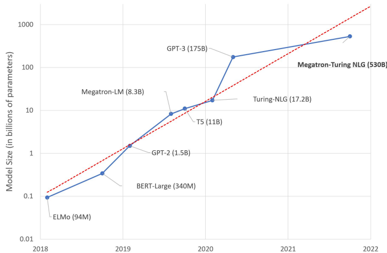
Figure 8.1: Evolution of the number of parameters for large language models. The figure is extracted from Microsoft blog post .
