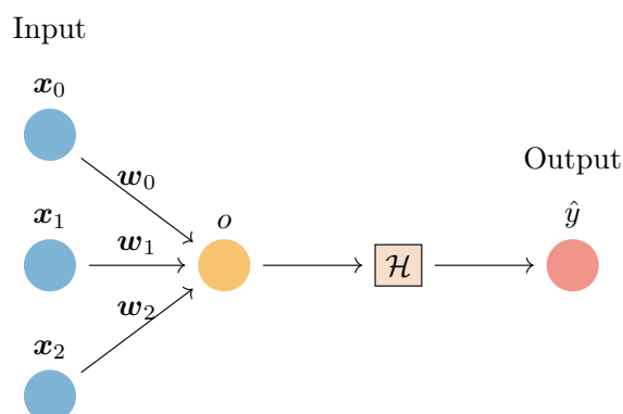
Figure 2.2: Perceptron.
