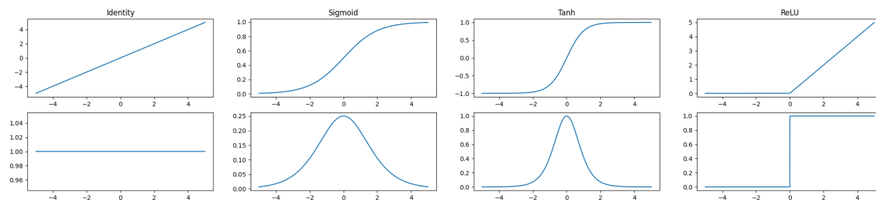
Figure 2.10: Activation functions (top) and their associated derivatives (bottom).
