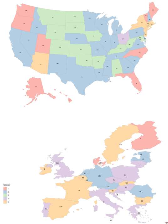
Figure 5.11: Clustering results.
