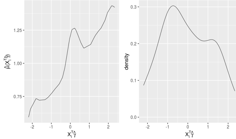
Figure 5.9: Estimator of the impact of the population risk factors \hat{\mu} (on the left) and density of the index X_i^T \hat{\gamma} (on the right).
