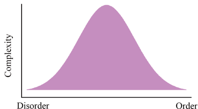
Figure 1C: The possible continuum of the complexity evolution. X-axis represents the evolution of the complexity from disorder (low predictability) to order (high predictability). Y-axis represents the level of complexity. An optimal complexity is at the top of the curve. Adapted from Stergiou & Decker (2011).
