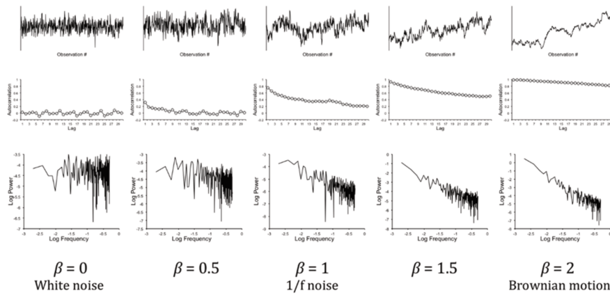
Figure 11: Distinction between White noise, 1/f noise and Brownian motion. From the White noise (left) to the Brownian motion (right), correlations in time series increased as reflect by the auto-correlation plots (middle) and the Log Power spectrum density (below). 1/f noise (pink noise, fractal time series) is represented in the middle column. This figure is extracted from Delignières & Marmelat (2012).
