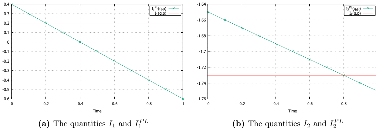
Figure VI.2: Simulations of the Peng-Luo's quantities and our first integrals
