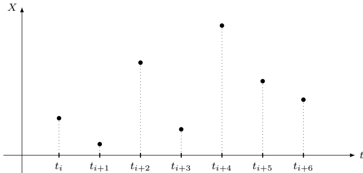
Figure II.1: A discrete function
