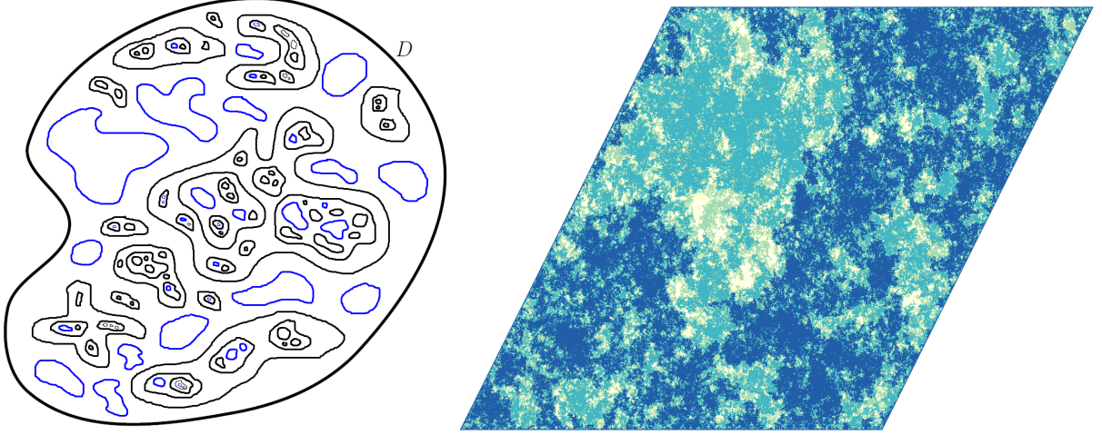
Figure 4.1: On the left: construction of the FPS of level -2\lambda through the nested \text{CLE}_4 . The blue loops correspond to the level -2\lambda and one does not iterate inside. On the right: computer simulations of FPSs of levels -\lambda (dark blue), -2\lambda , -3\lambda and -4\lambda (bright yellow). Done with the help of Brent Werness.
