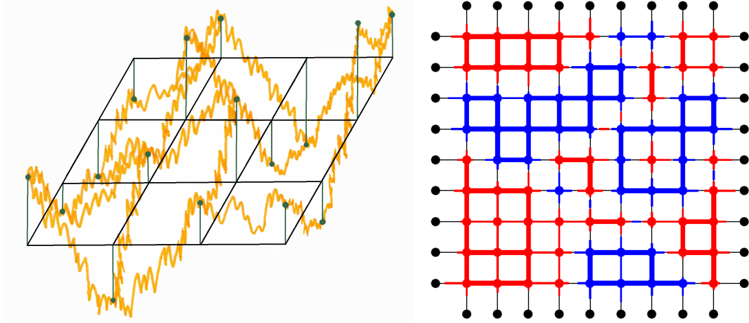
Figure 3.1: On the left, an illustration of the metric graph GFF. In green is the height of the discrete GFF on the vertices. In orange the interpolating Brownian bridges. On the right, the sign clusters of metric graph GFF, positive in red and negative in blue. The bold lines represent the edges visited by the random walk loops. The black dots represent the boundary vertices in V_\partial . The boundary condition is 0.
