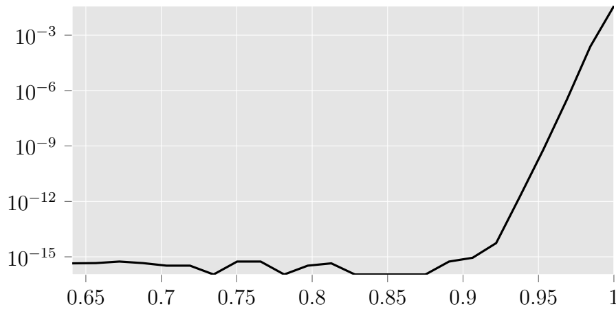
Figure 8.12: Plot of the terminal error using the update initialisation technique. Abscissa is 10^3\lambda and the y-axis is the log-norm of the endpoint error e_\lambda(1) . The solid black line shows the evolution of the log-norm \log(\|e_\lambda(1)\|) against \lambda with updated initialisation at every \lambda .
