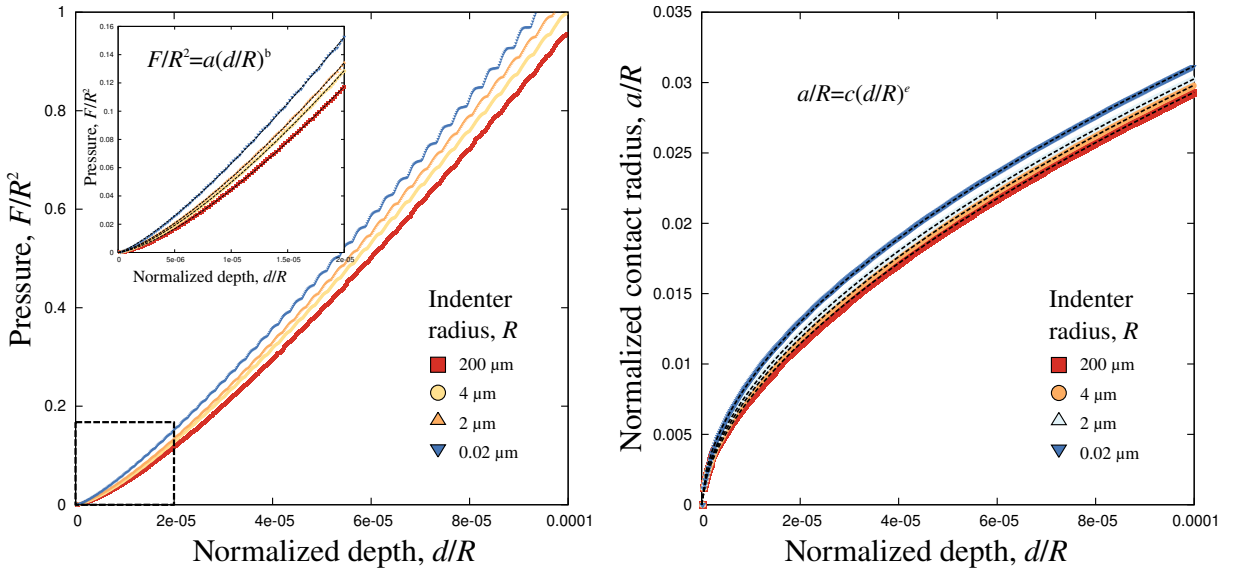
Figure 1.18: Normalized force-penetration and radius-penetration for a spherical indenter using Cosserat continuum.
