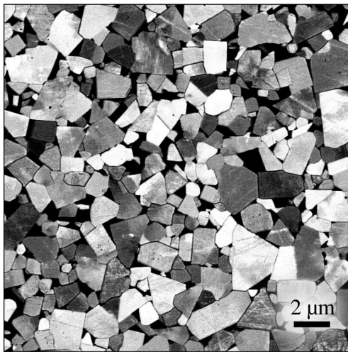
WC/Co microstructure (SEM)
